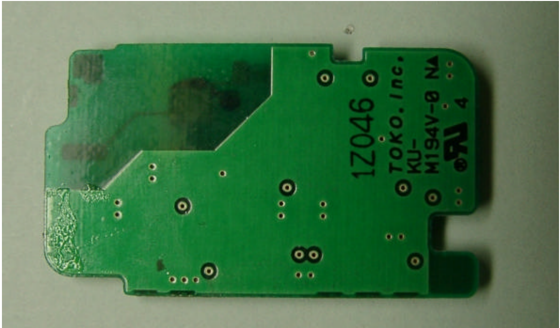
INVERTER TRANSFORMER LCD BOTTOM
