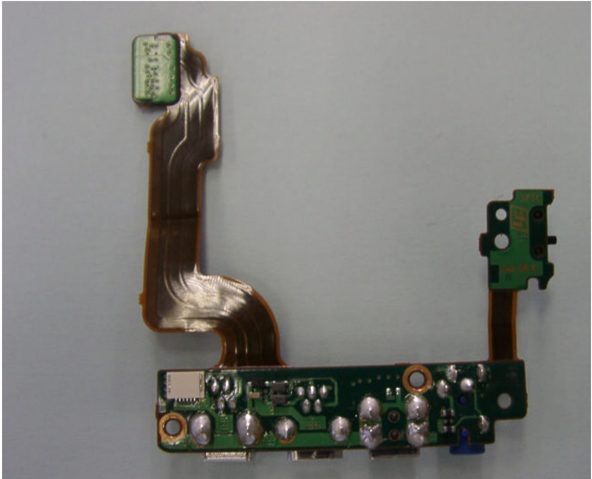
JACK BOTTOM
