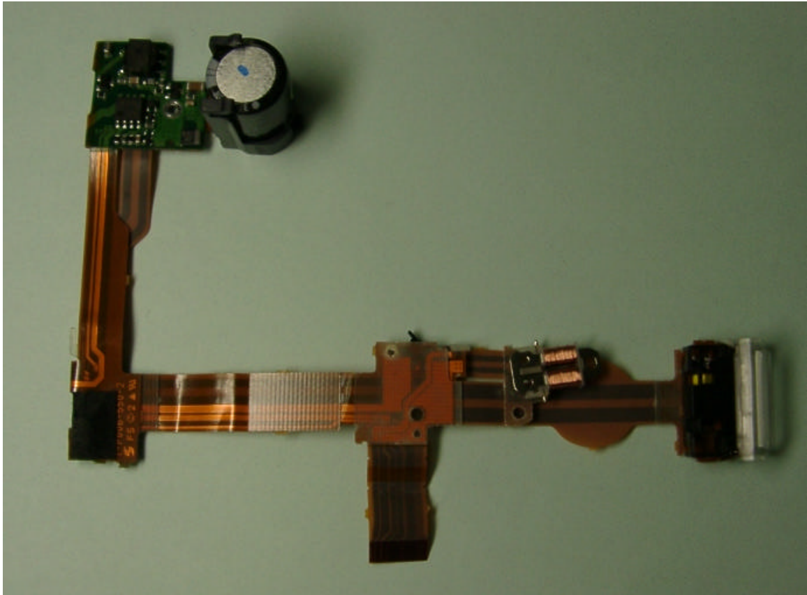
FLASH UNIT ONE BOTTOM
