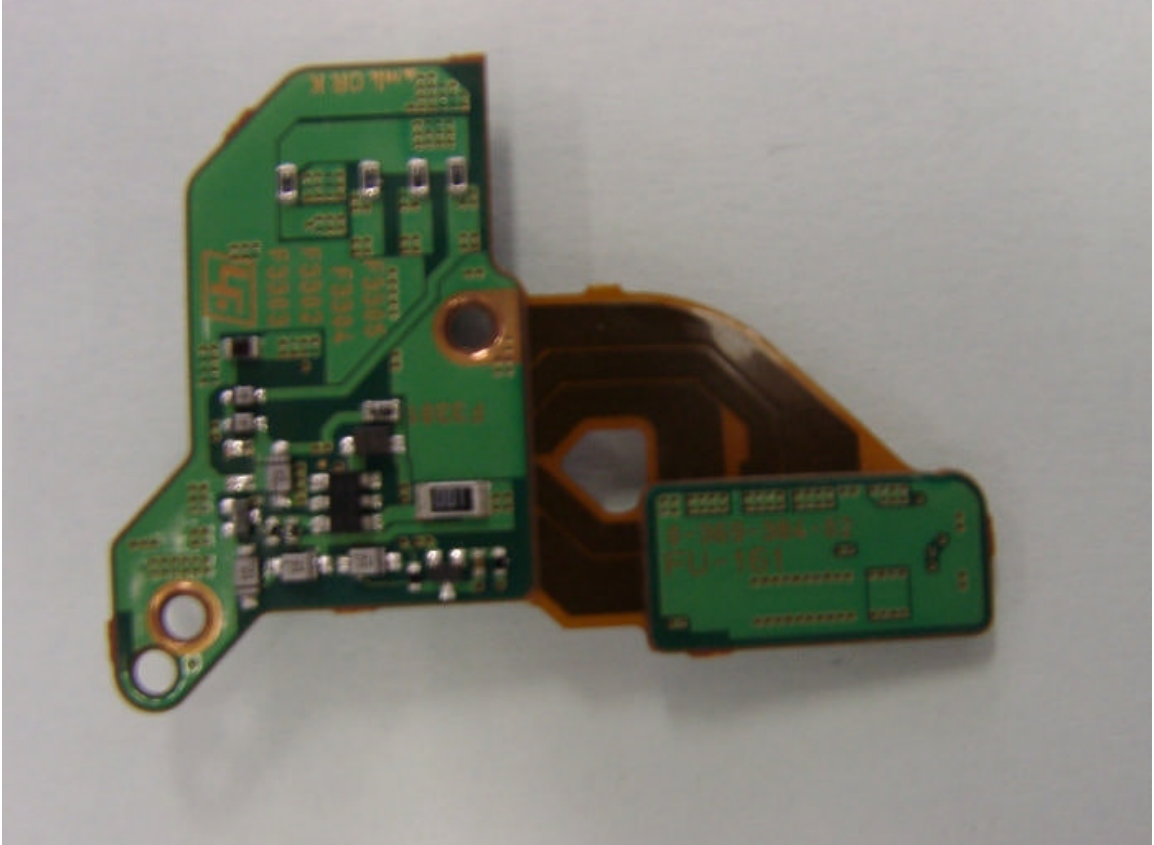
FUSE BOTTOM
