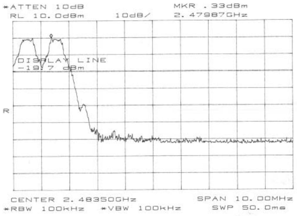
figure 18 Band Edge High frequency side
