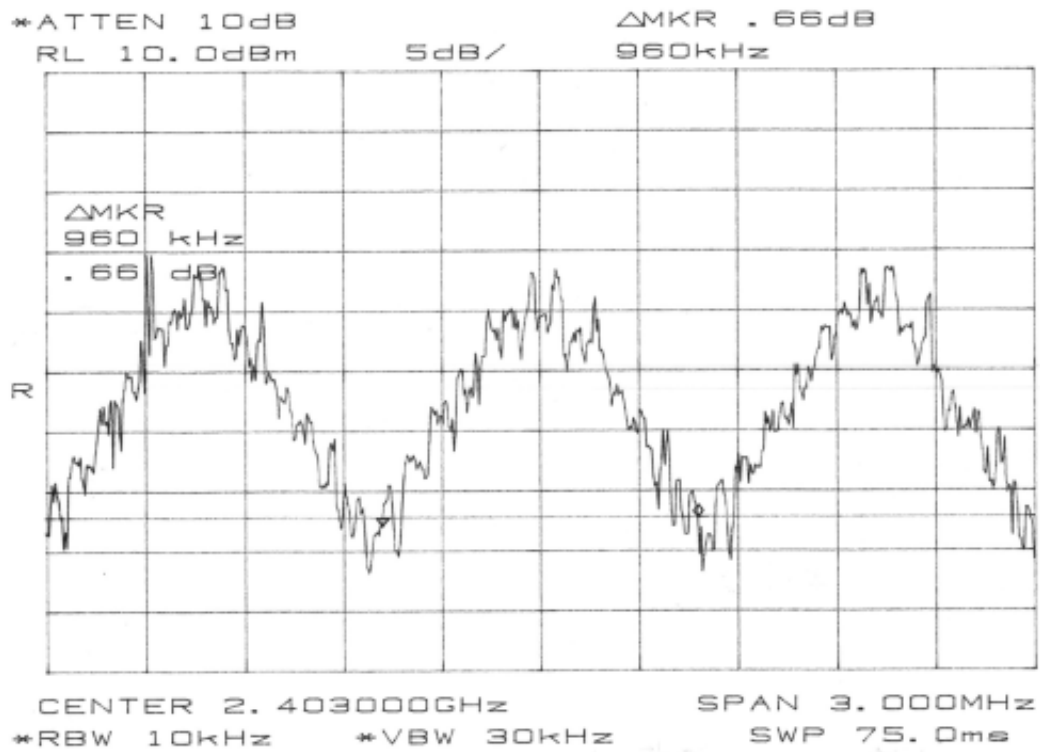
figure 11 20dB Bandwidth f_c = 2403 MHz
