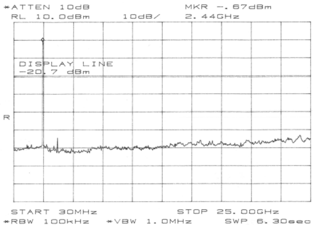
figure 20 Spurious RF conducted emission, Tx on 2441 MHz
