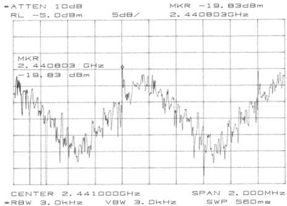
figure 23 Power Density, Tx on channel 20
