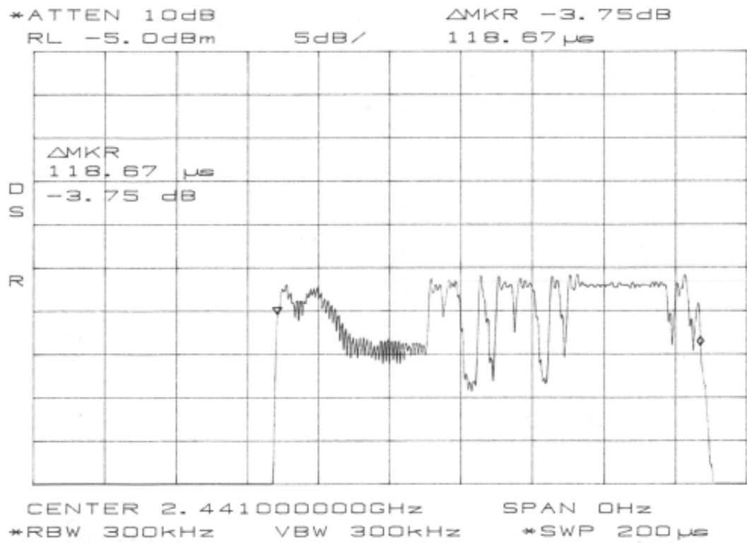
figure 7 Duration of one transmission
