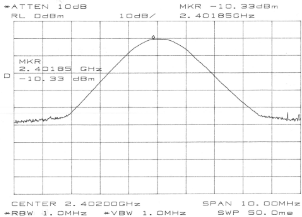
figure 14 2402 MHz (channel 2)
