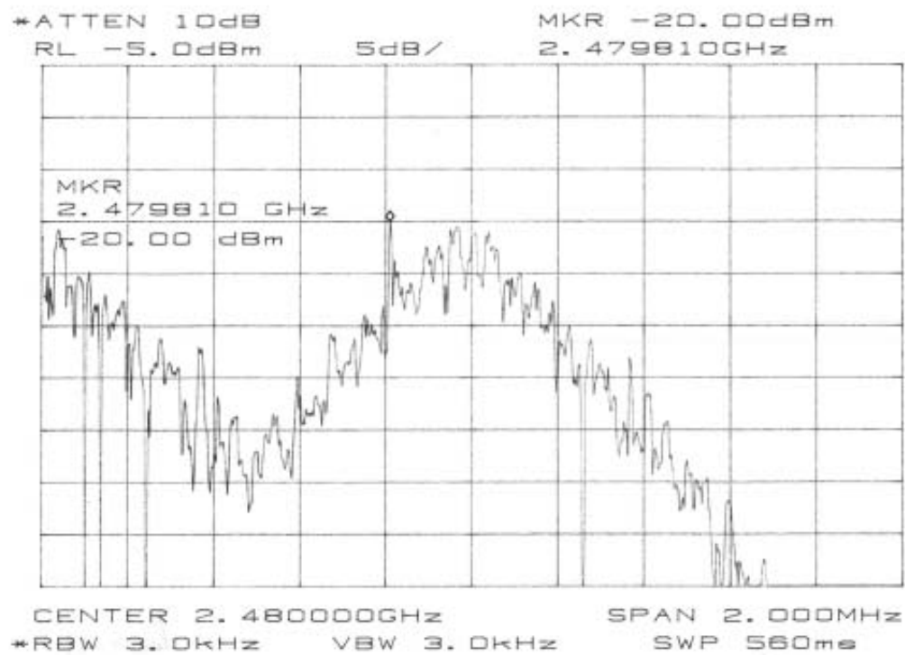
figure 24 Power Density, Tx on channel 80
