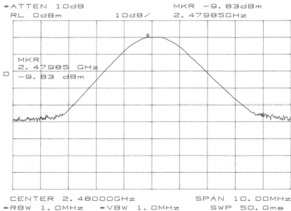
figure 16 2480 MHz (channel 80)
