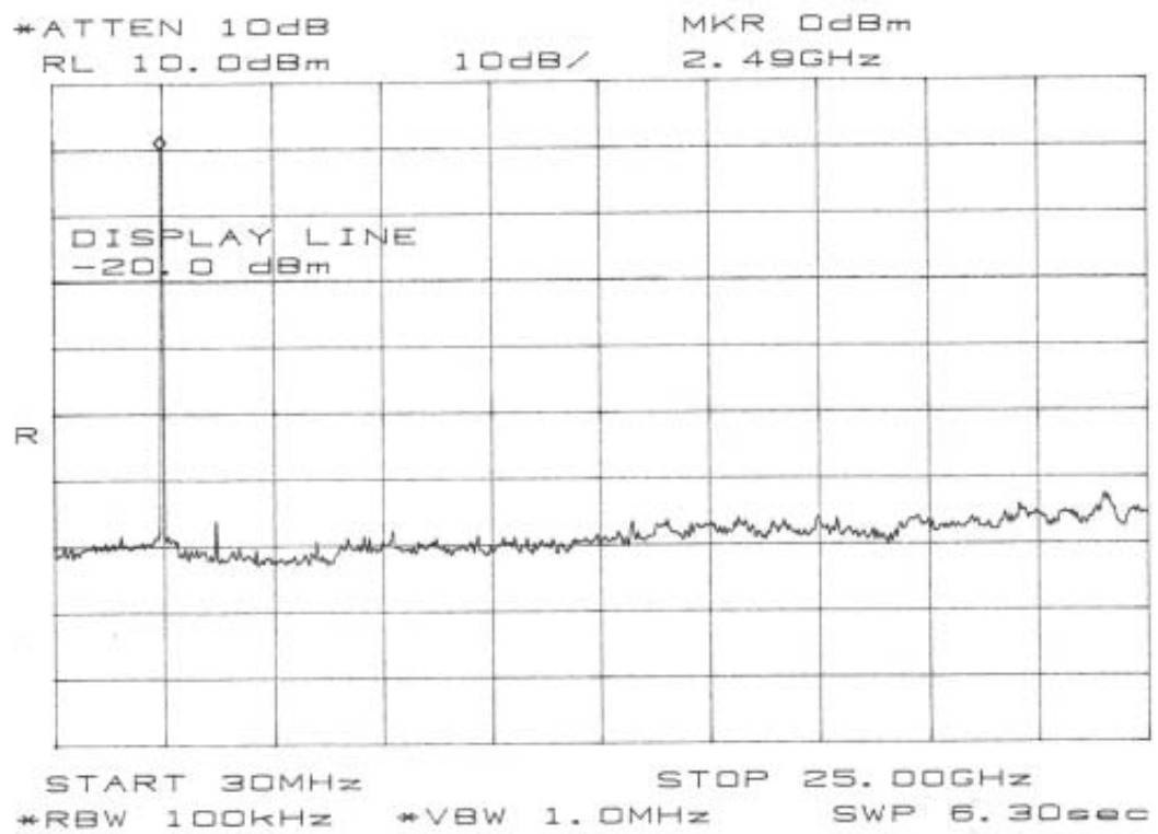
figure 21 Spurious RF conducted emission, Tx on 2480 MHz
