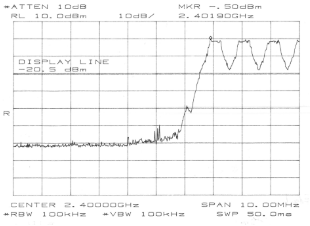
figure 17 Band Edge Low frequency side
