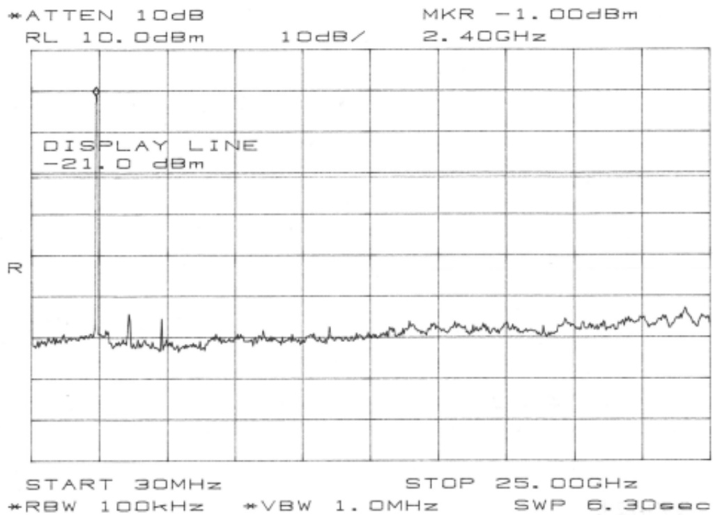
figure 19 Spurious RF conducted emission, Tx on 2402 MHz
