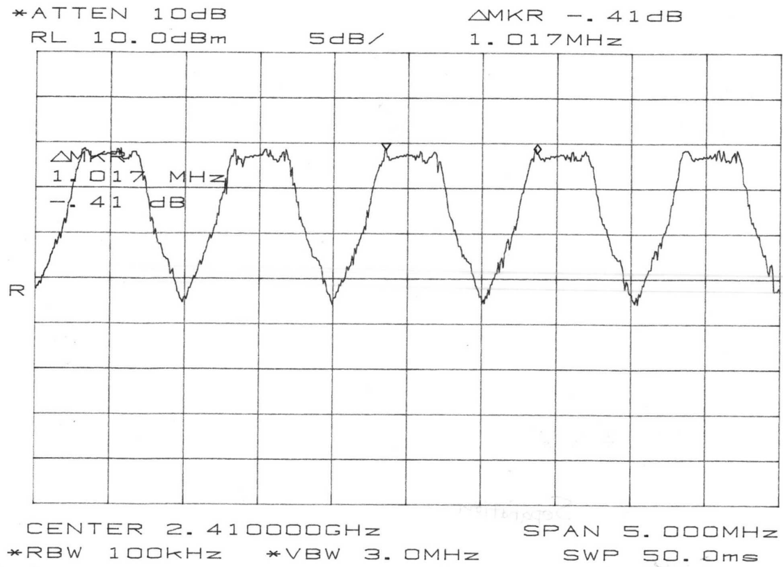
figure 1 Carrier frequency Separation f_c = 2410 MHz
