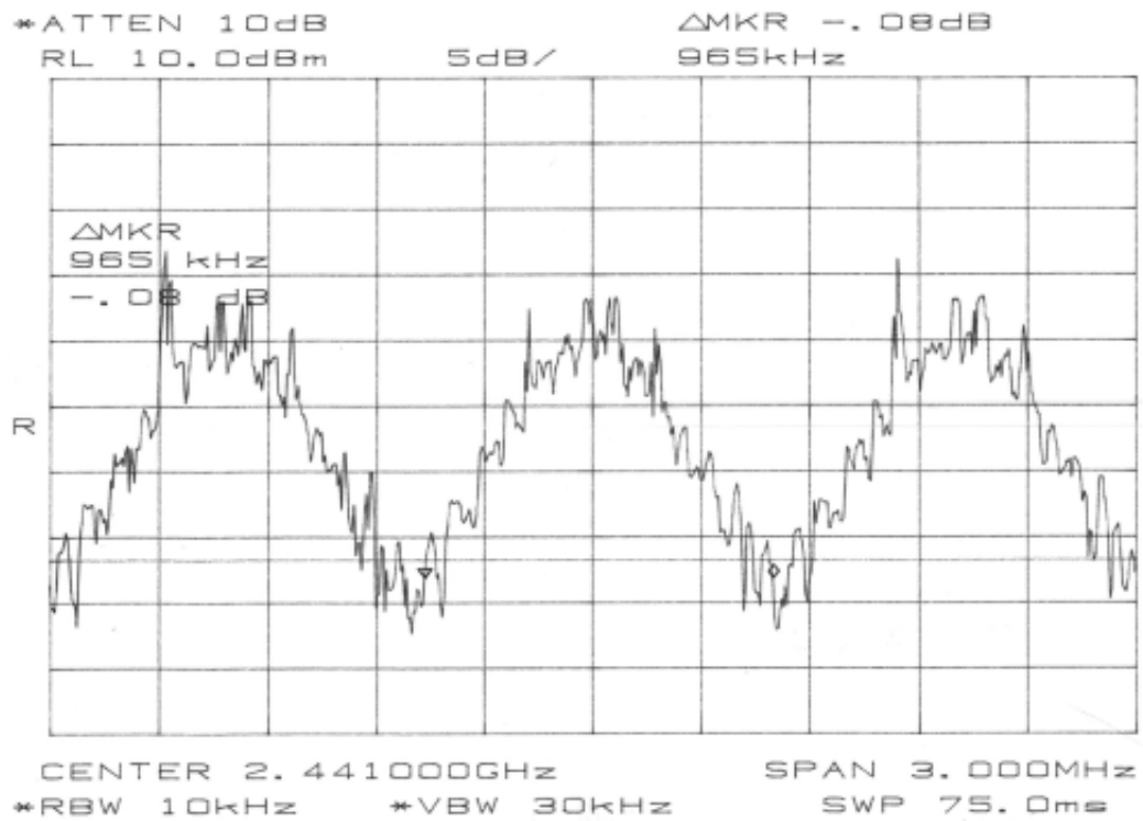
figure 12 20dB Bandwidth f_c = 2441 MHz
