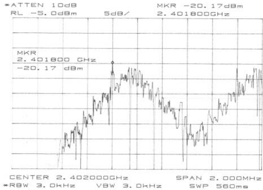
figure 22 Power Density, Tx on channel 2
