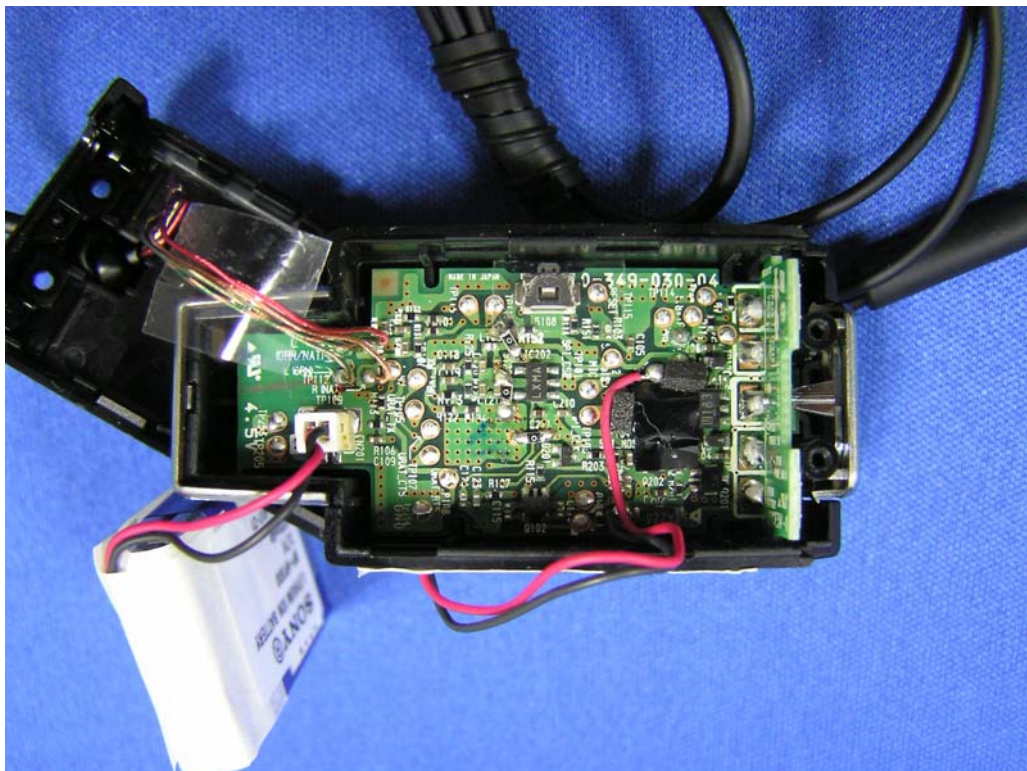
Soldering Side
