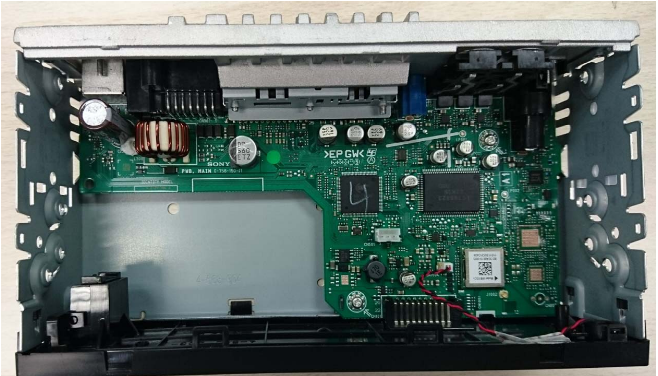
Main side
