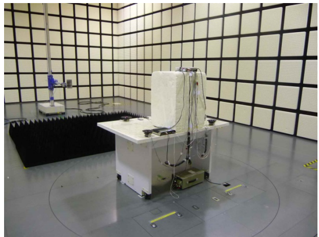
Above 1 GHz
