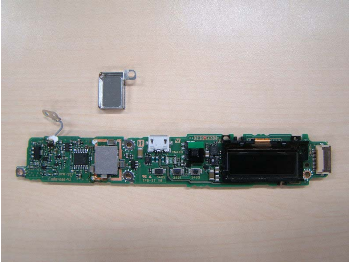
Fig.23: Removed the shield case
