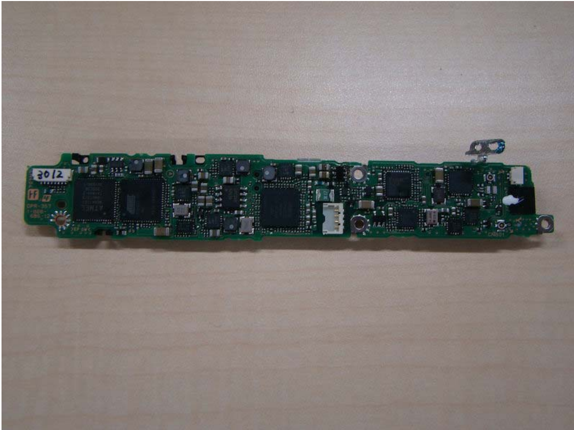
Fig.21: Side A of Board DPR-357
