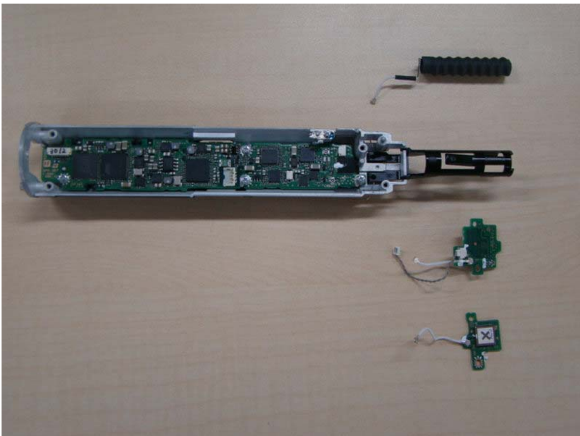
Fig.14: Removed the Antenna, Board RF-165, Board AN-38
