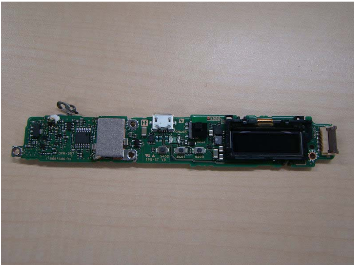
Fig.22: Side B of Board DPR-357
