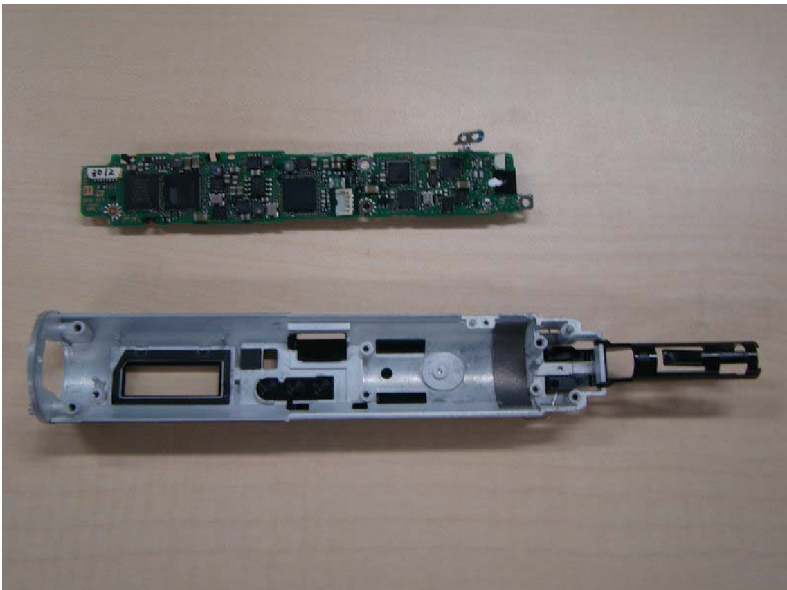
Fig.20: Removed the Board DPR-357
