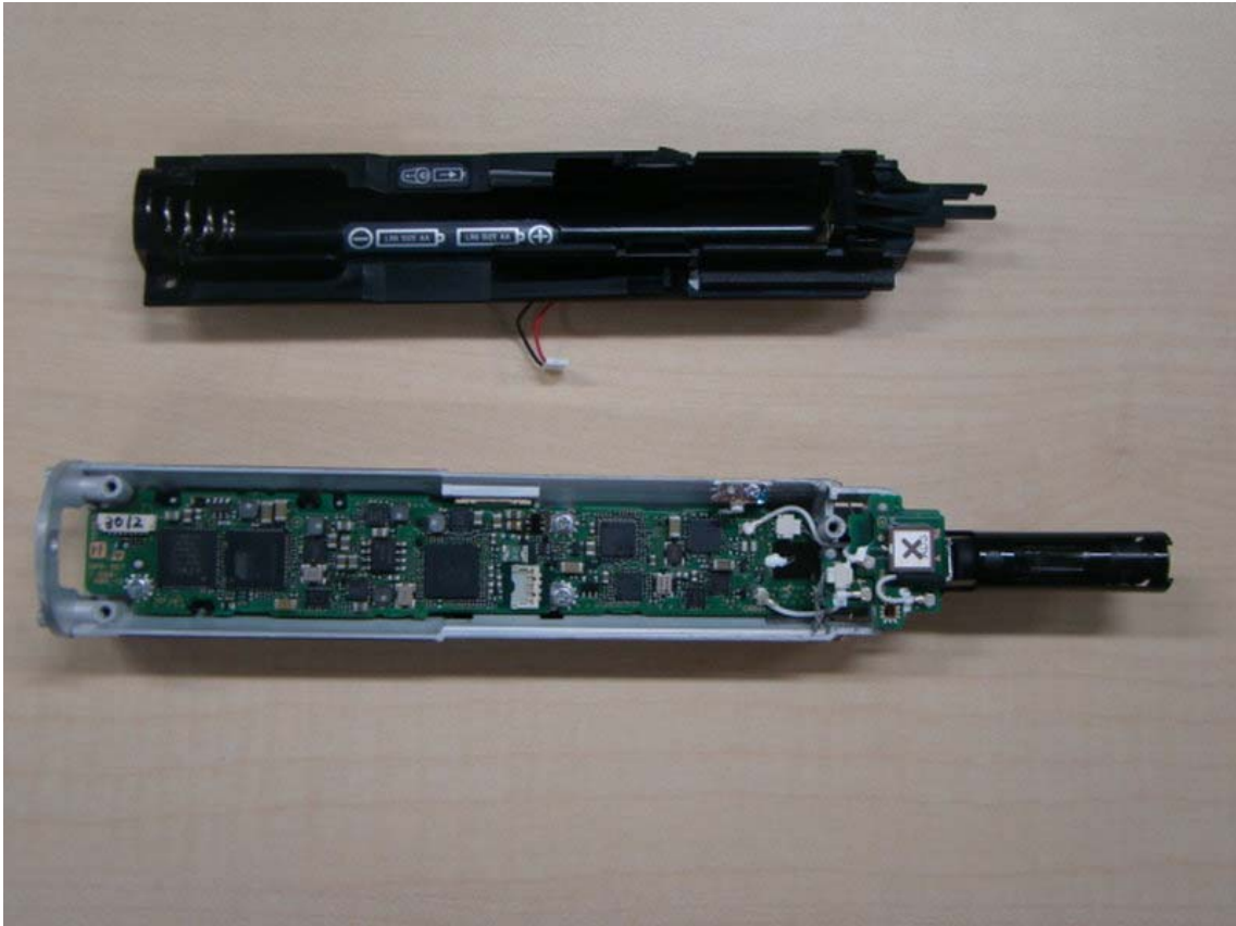
Fig.11: Removed the Battery case
