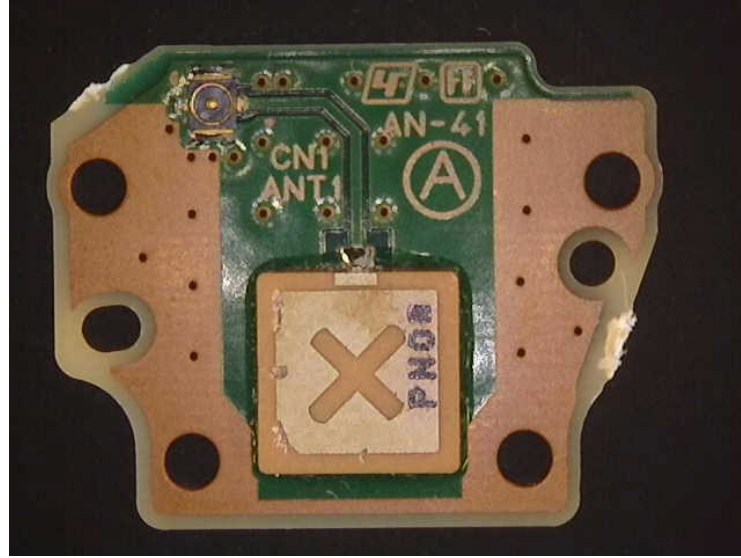
AU-395 Side A
