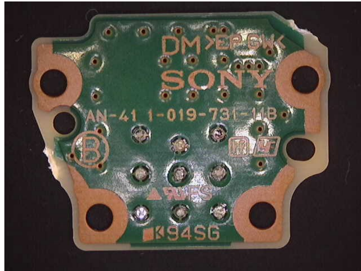
AU-395 Side B
