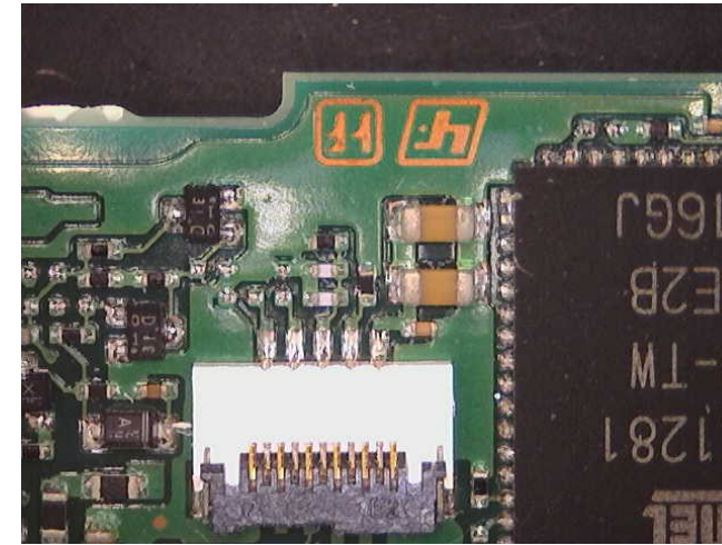
TX-182 Side B(without shield case)
