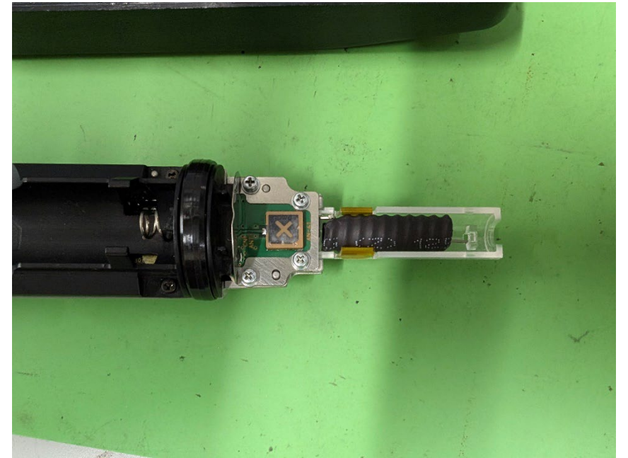
Antenna Under Test
