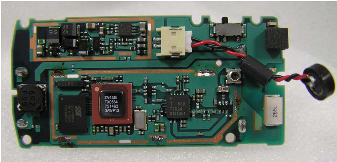
Side A (without Shield)
