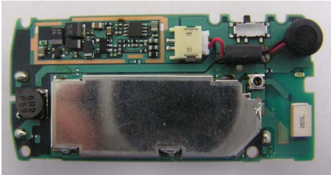
Side A (with Shield)
