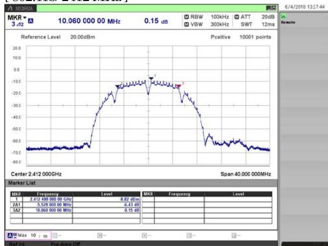
[ 802.11b/ 2412 MHz ]
