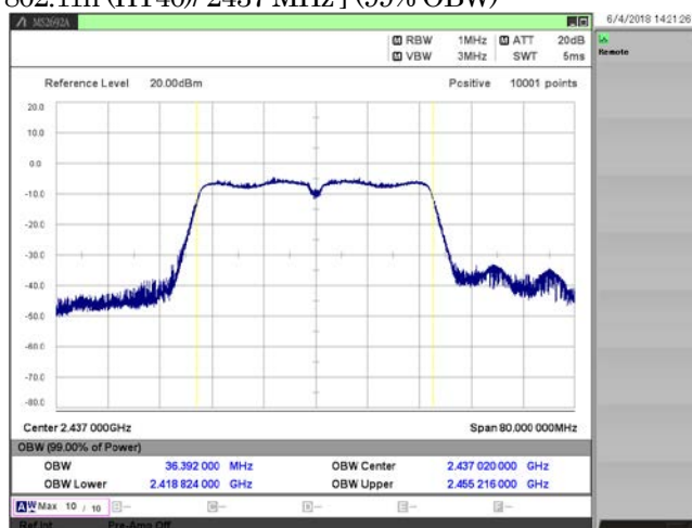
[ 802.11n (HT40)/ 2437 MHz ] (99% OBW)
