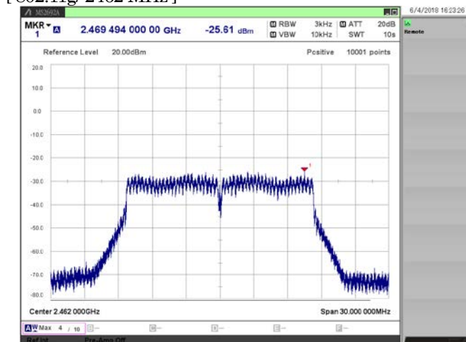
[ 802.11g/ 2462 MHz ]
