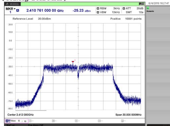
[ 802.11g/ 2412 MHz ]
