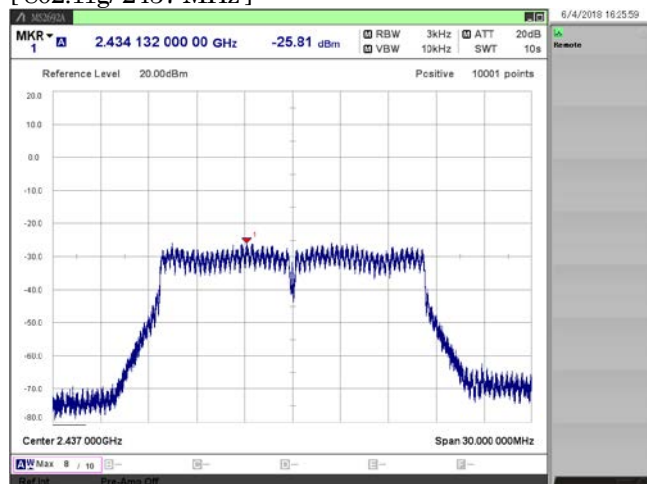
[ 802.11g/ 2437 MHz ]
