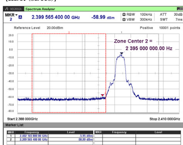
[EDR (3DH5)]
