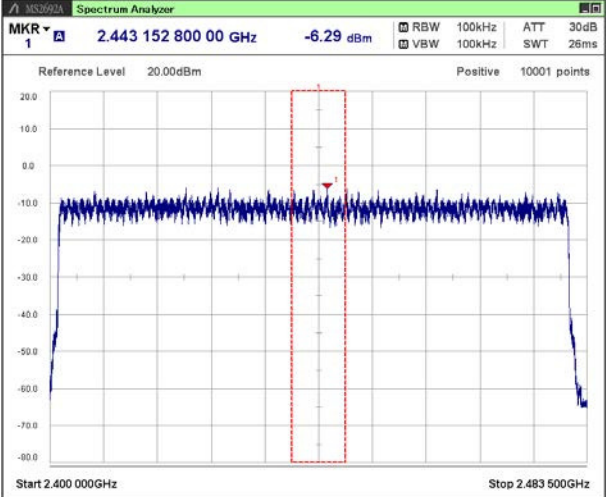
[EDR (3DH5)]
