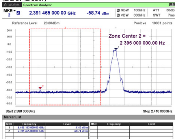
[BDR (DH5)]
