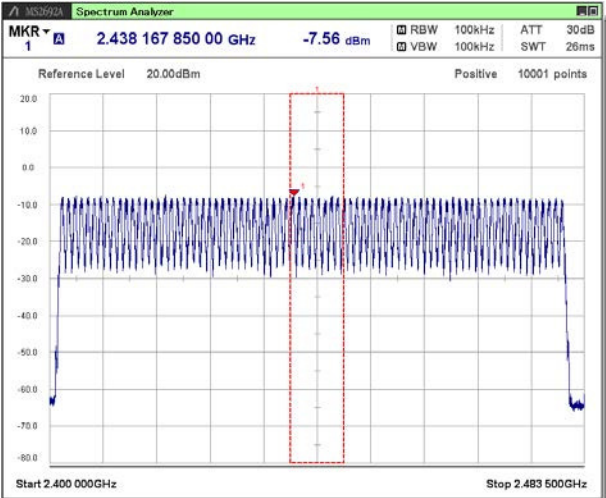
[BDR (DH5)]
