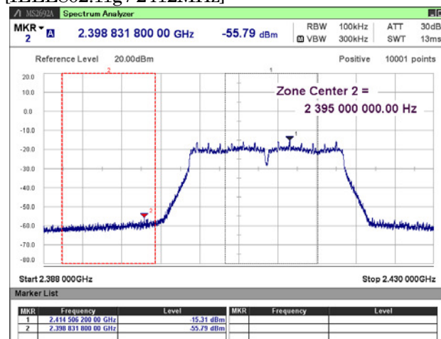
[IEEE802.11g / 2412MHz]
