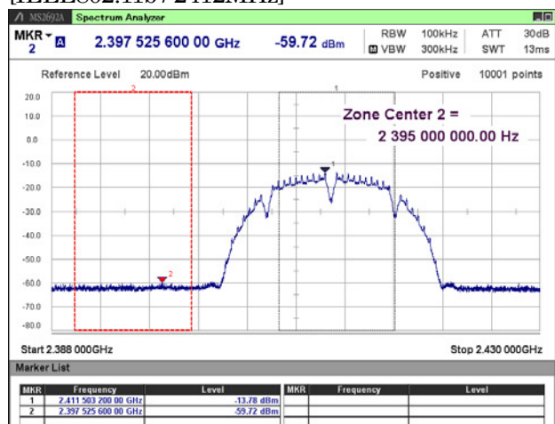
[IEEE802.11b / 2412MHz]
