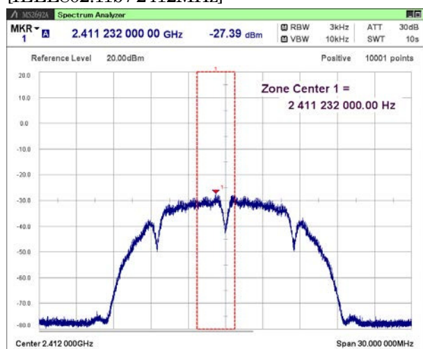
[IEEE802.11b / 2412MHz]
