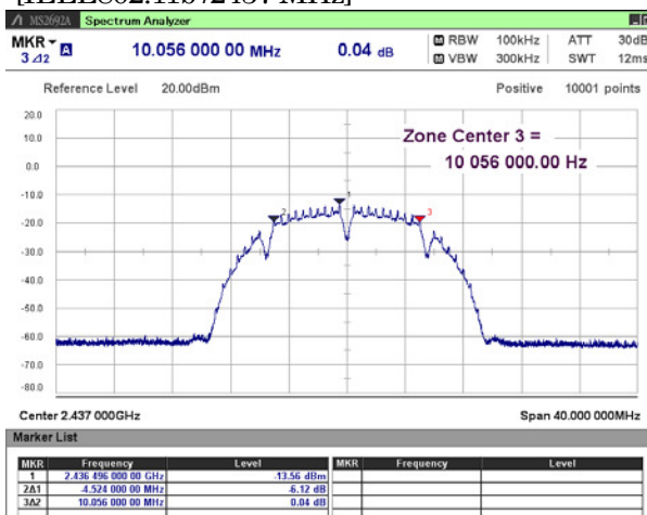
[IEEE802.11b / 2437 MHz]
