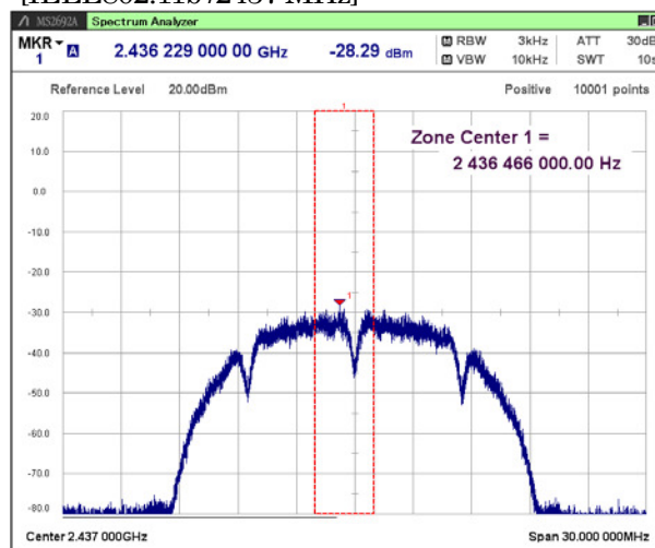
[IEEE802.11b / 2437 MHz]
