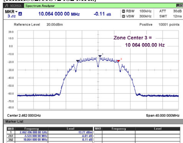
[IEEE802.11b / 2462 MHz]
