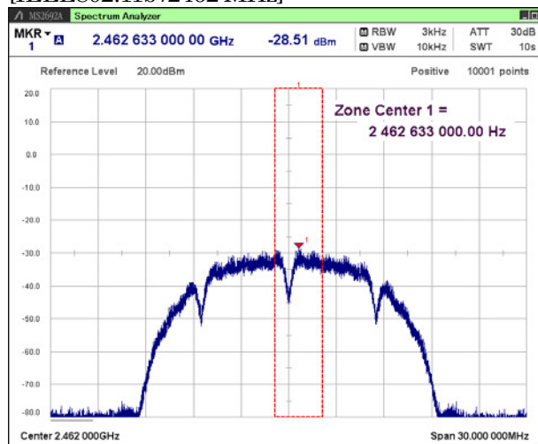
[IEEE802.11b / 2462 MHz]
