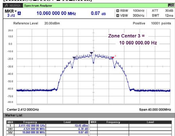
[IEEE802.11b / 2412MHz]
