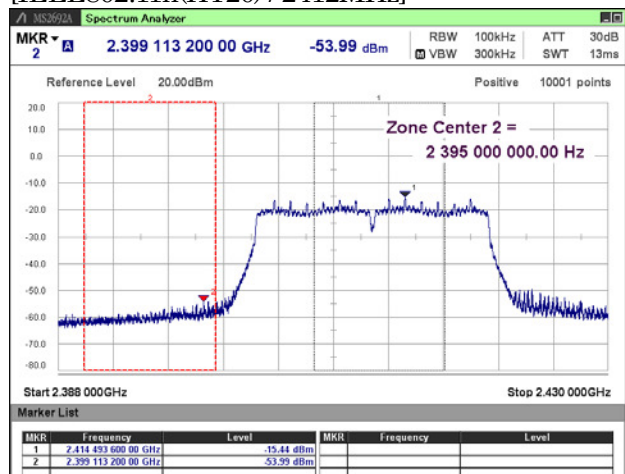
[IEEE802.11n(HT20) / 2412MHz]
