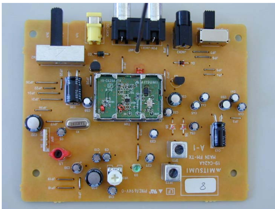
Module front (Not Shielded)
