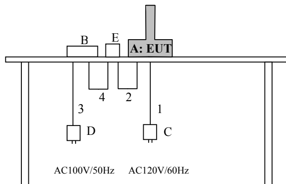
Top View (Radiated emission)
