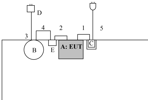
Top View (Conducted emission)
