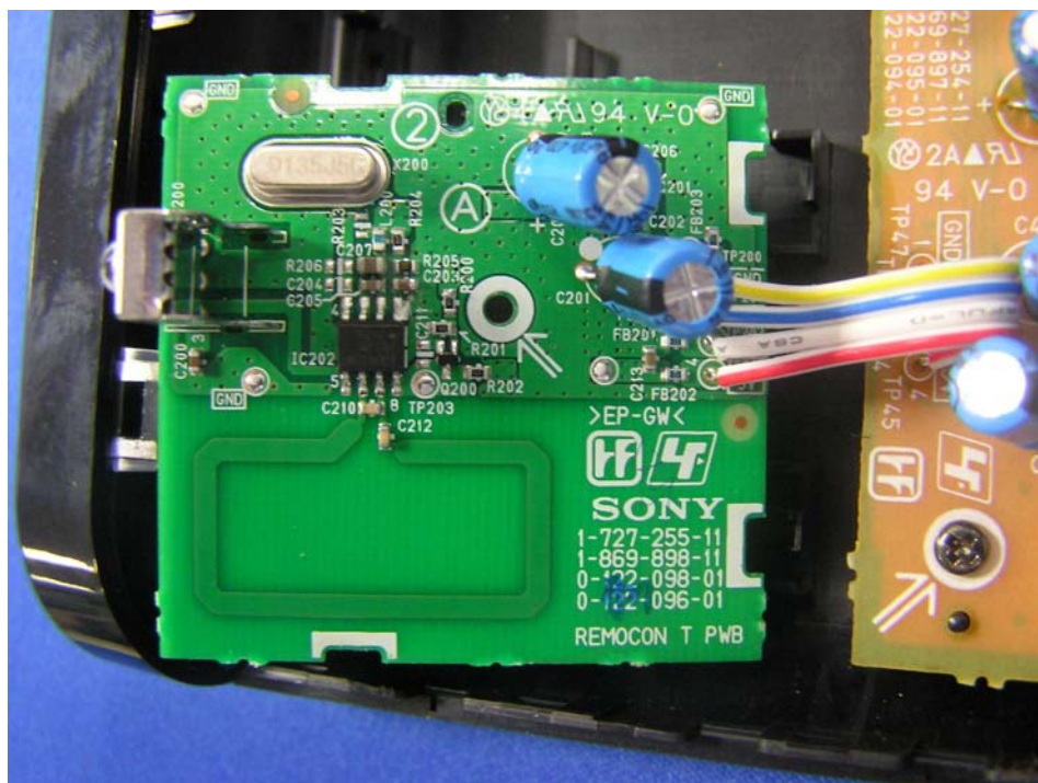
433MHz TX PCB Assy (Top)
