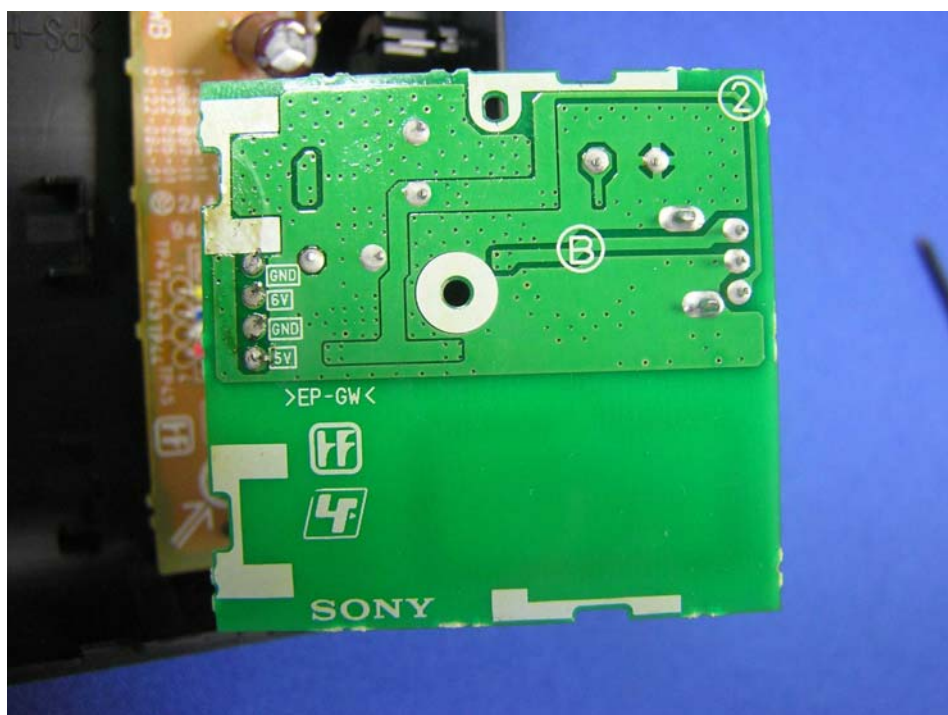
433MHz TX PCB Assy (Bottom)
