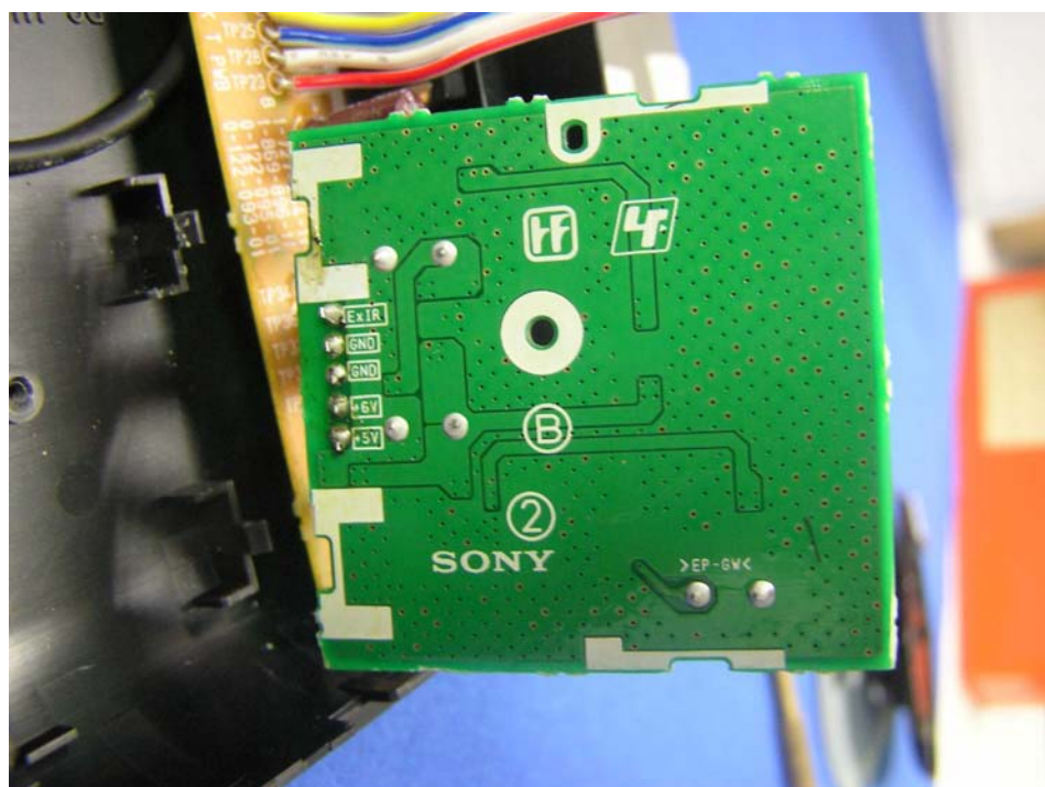
433MHz RX PCB Assy (Bottom)
