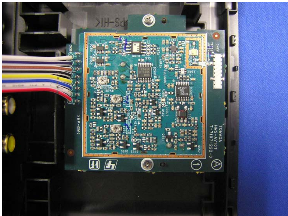
2.4GHz TX Module (Top)
