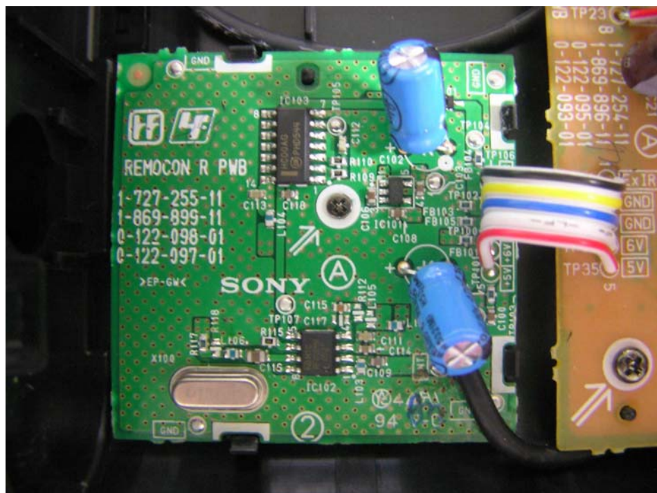
433MHz RX PCB Assy (Top)
