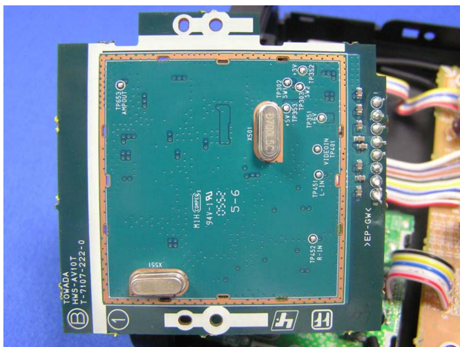
2.4GHz TX Module (Bottom)
