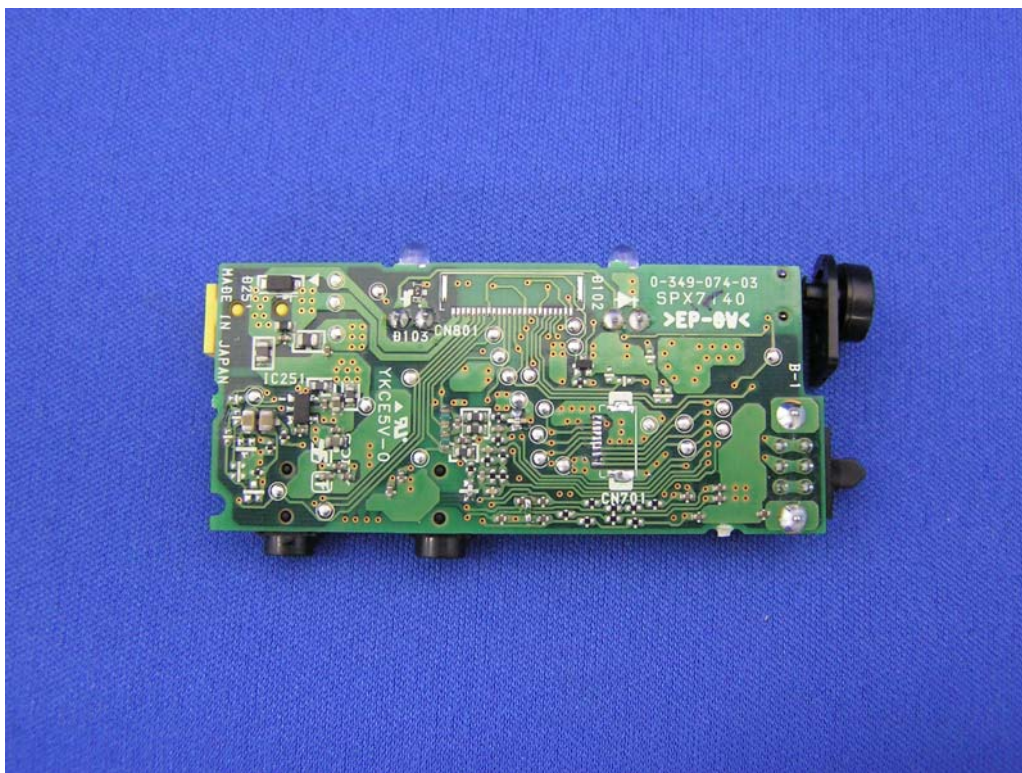
Soldering Side
