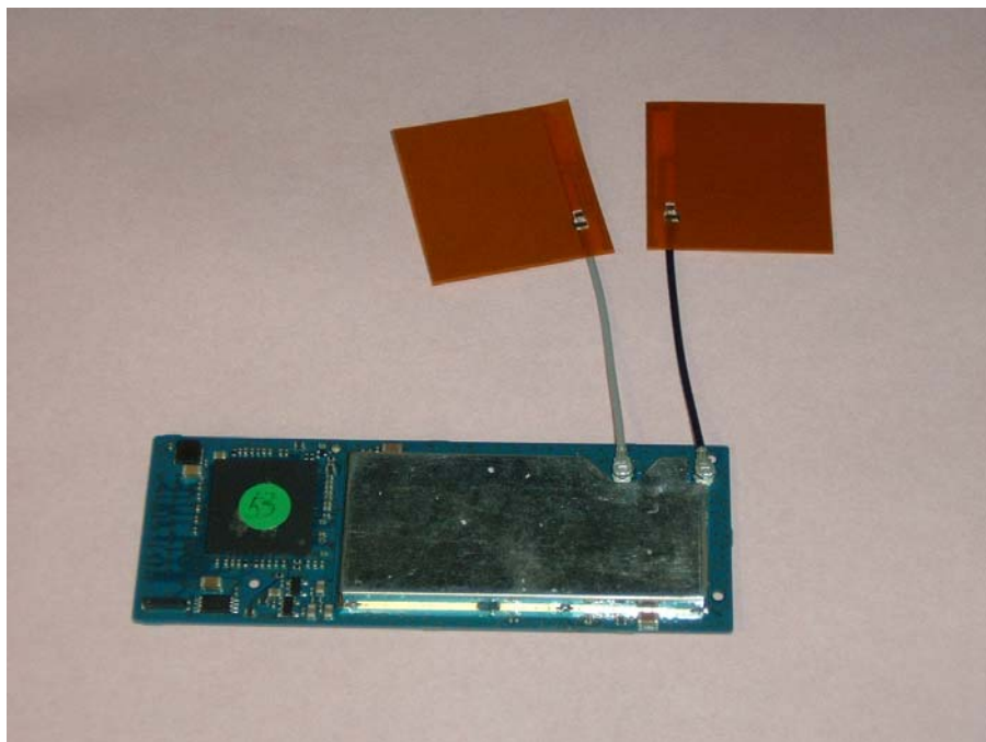
Front View of Wireless LAN Module with Antenna (HFT18) and Shielding
