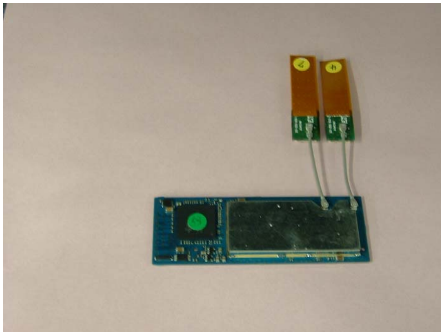
Front View of Wireless LAN Module with Antenna (EA5800) and Shielding
