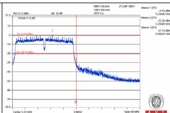
EUT (Client) links with master on 11ac (VHT40) mode
