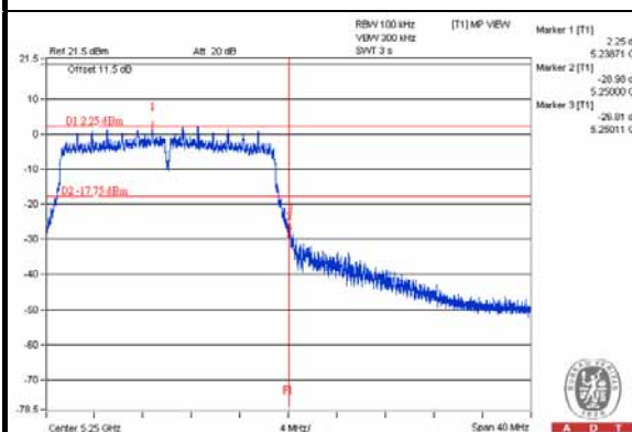
EUT (Client) links with master on 11ac (VHT20) mode
