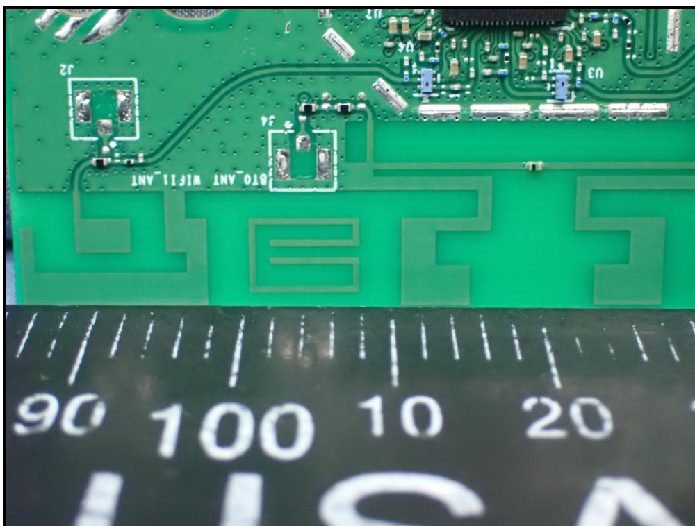
Antenna_BT 0
