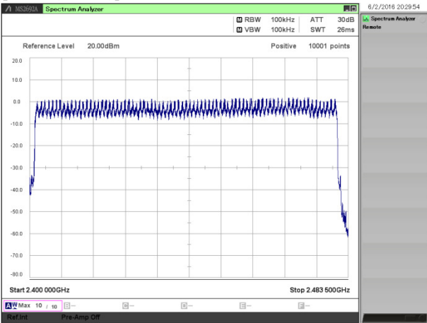
[EDR (3DH3)]
