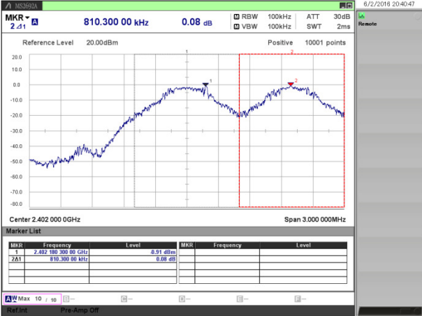
[BDR (DH5)]
