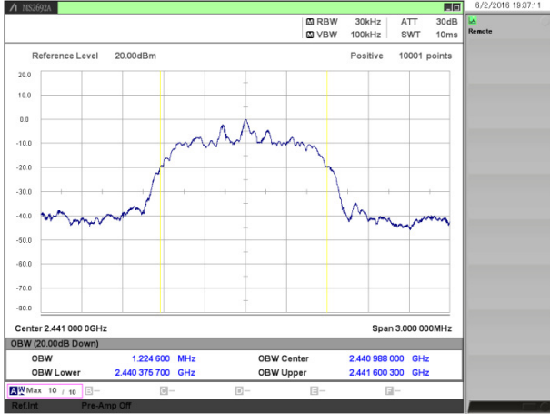
[EDR (3DH3) / 2441MHz]
