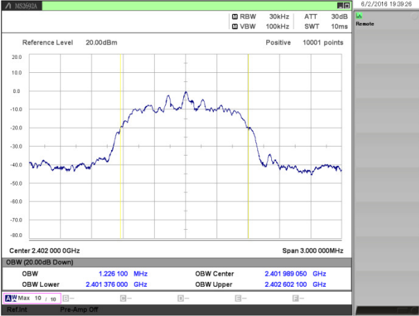
[EDR (3DH3) / 2402MHz]
