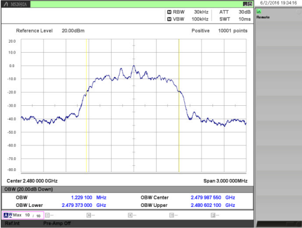
[EDR (3DH3) / 2480MHz]
