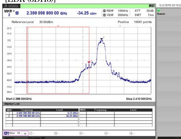
[EDR (3DH3)]
