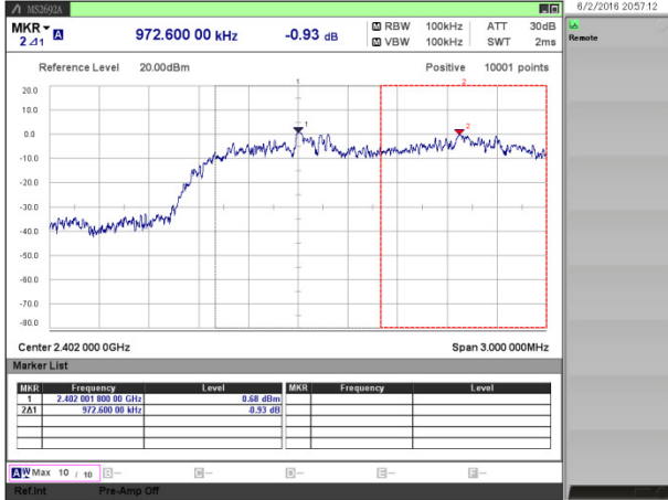
[EDR (3DH3)]
