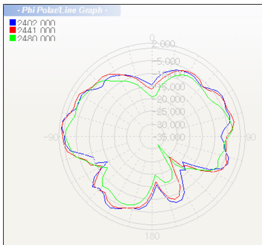
(c) Elevation2 Plane (XZ)
