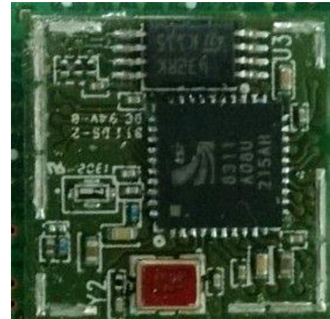
Internal BT module Without shield case
