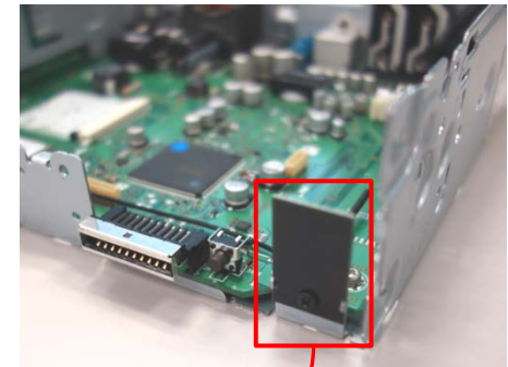
BLUETOOTH Antenna
