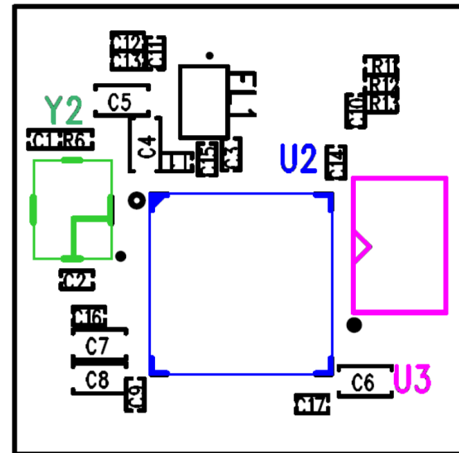
Parts mounting diagrams
