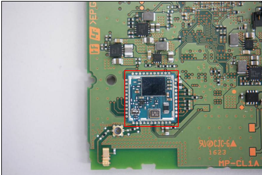
View of Bluetooth, WLAN antenna
