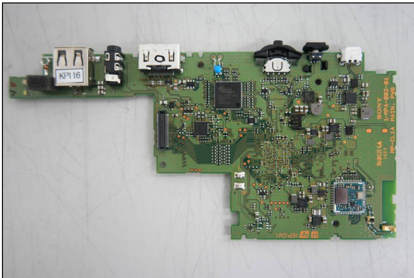
Top view of Main PCB (Shielding off)
