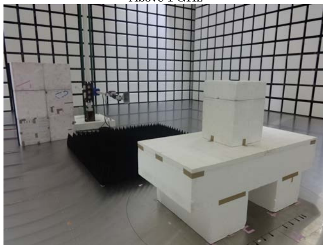
Above 1 GHz
