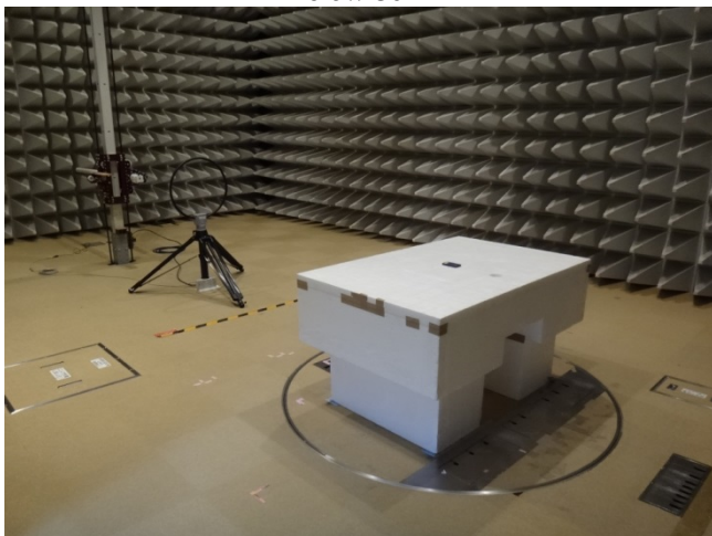
Below 30MHz
