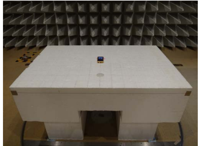
30 - 1000 MHz
