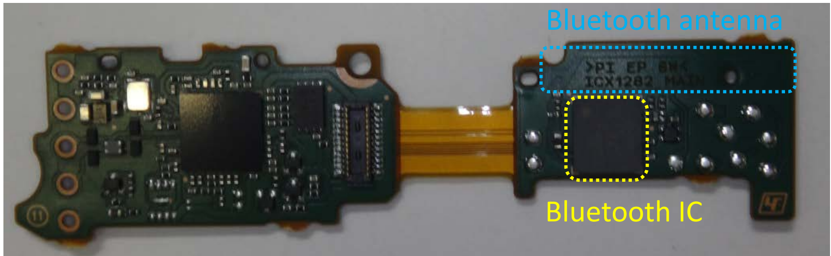
Main PWB-Bottom
