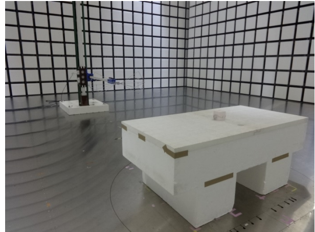
30 - 1000 MHz
