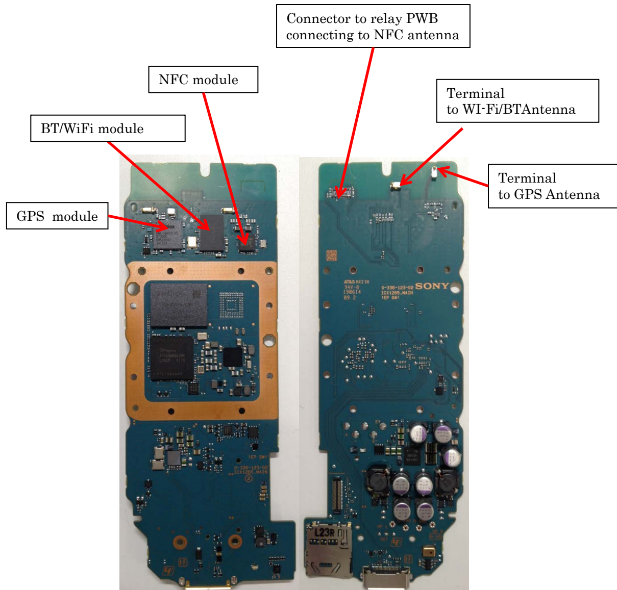
PWB Top view
