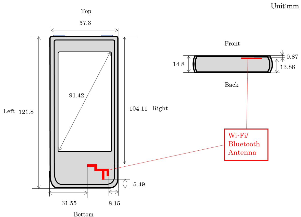
Figure D-4 Antenna Dimensions and Separation Distances
