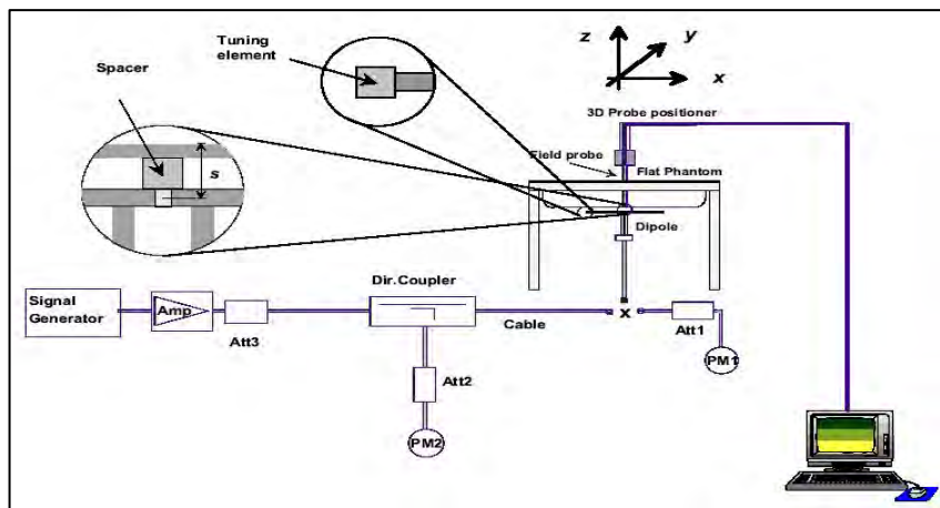
Test setup for the system performance check
