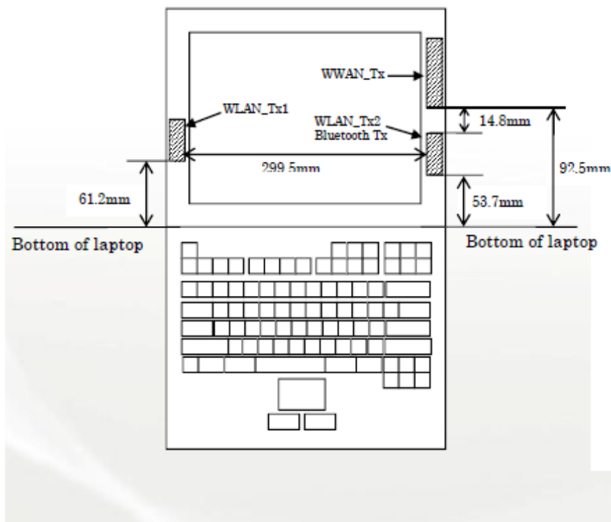
Figure 11-2 Antenna Diagram
