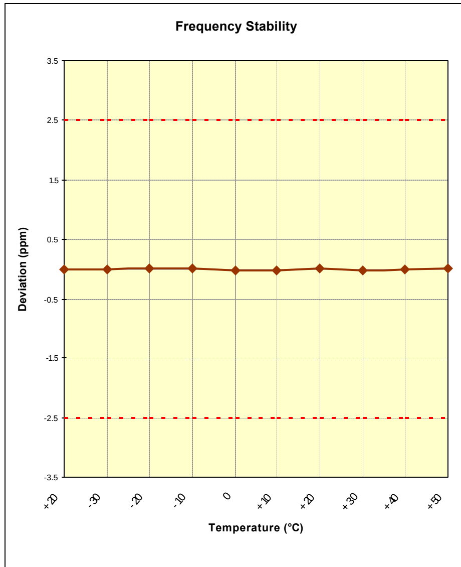
Figure 6-4. Frequency Stability Graph (PCS GSM Mode – Ch. 661)
