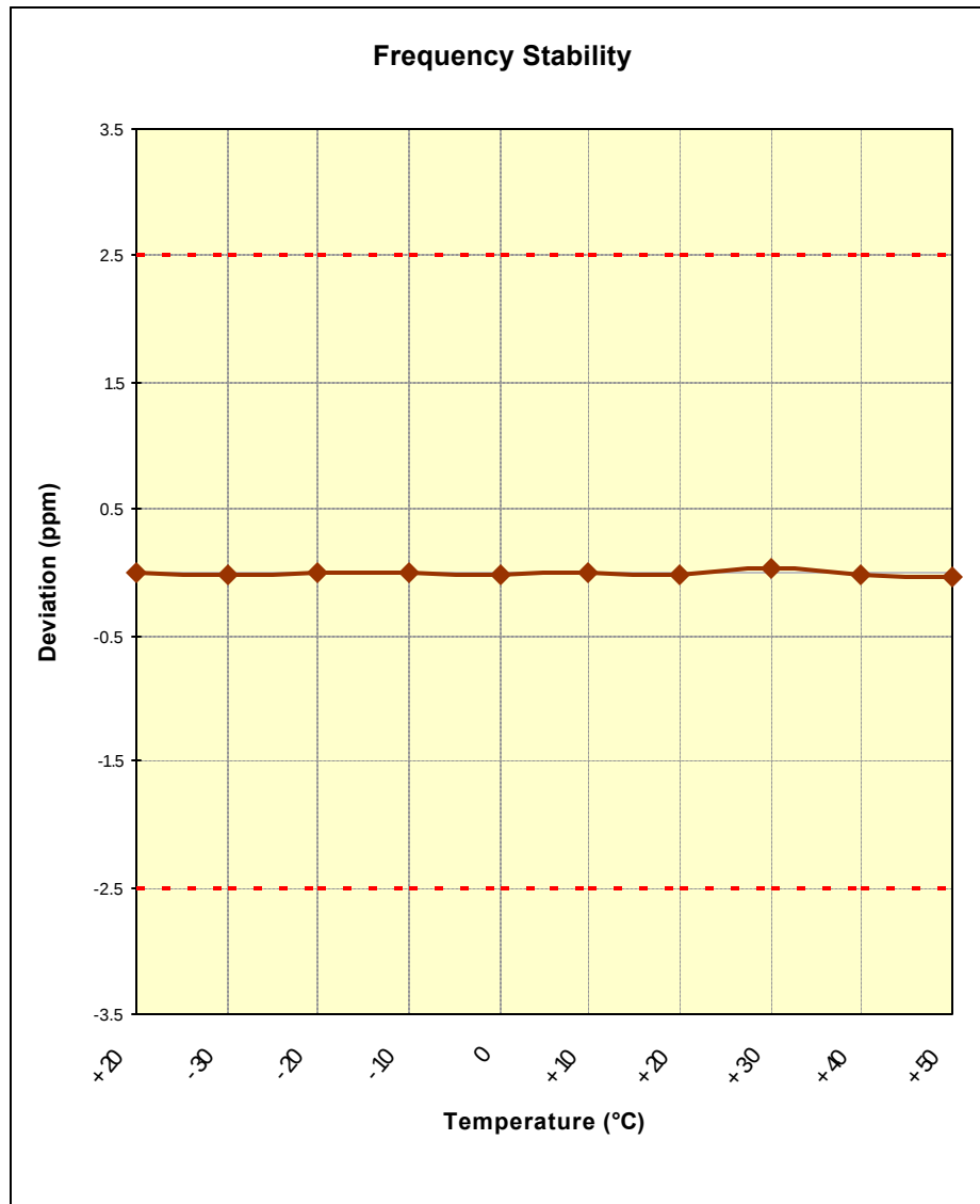
Figure 6-3. Frequency Stability Graph (Cellular CDMA Mode – Ch. 384)
