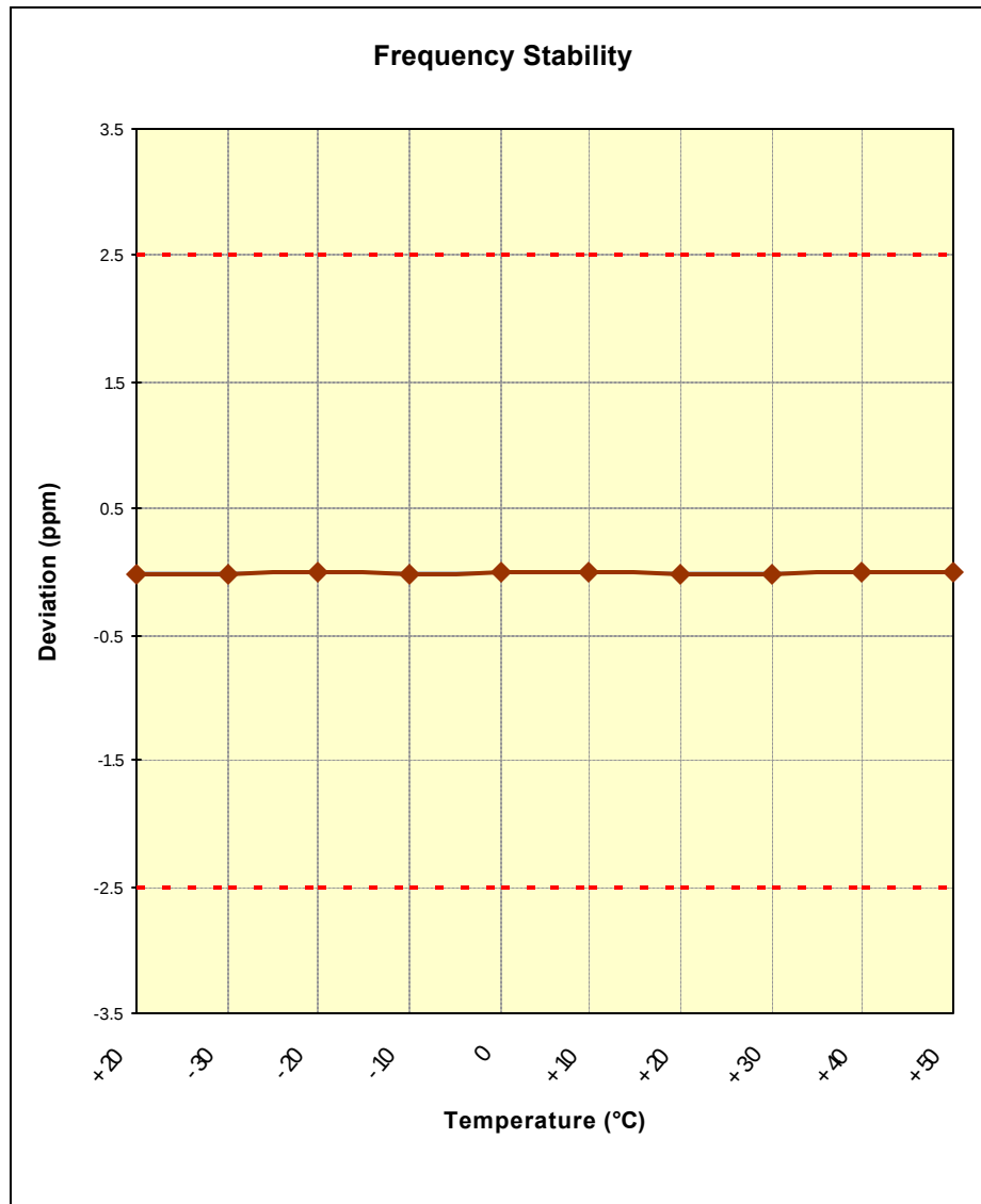
Figure 6-6. Frequency Stability Graph (PCS CDMA Mode – Ch. 600)
