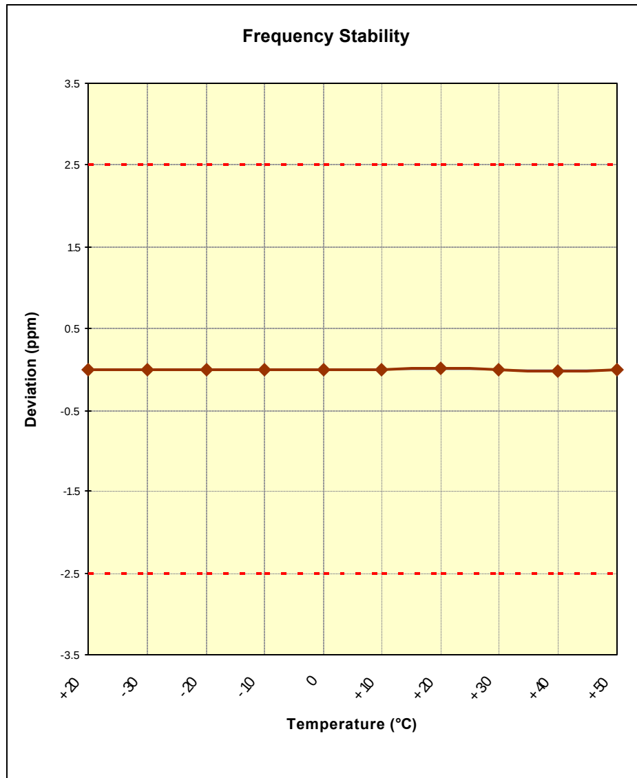
Figure 6-5. Frequency Stability Graph (PCS WCDMA Mode – Ch. 9400)
