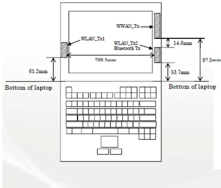
Figure 13-2 Antenna Diagram
