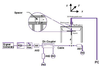
Figure 16-1 System Verification Setup Diagram
