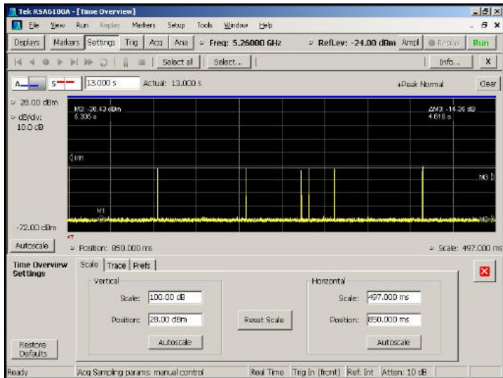
Figure 5-7. Traffic pulse grouping 1
