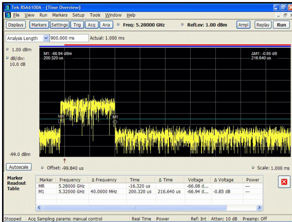
Figure 5-11. Pulse Width After 200ms
