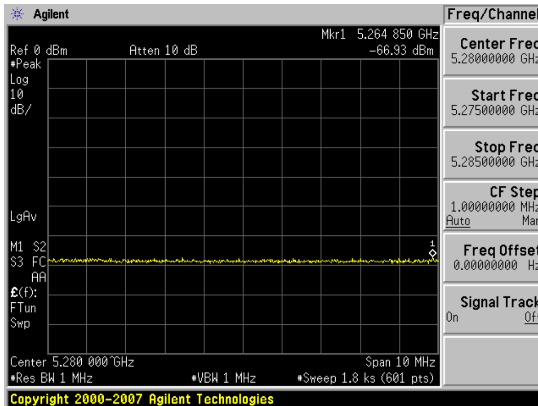
Figure 5-12 Non-occupancy Period - Monitoring live real time spectrum - Elapse time 30 minutes
