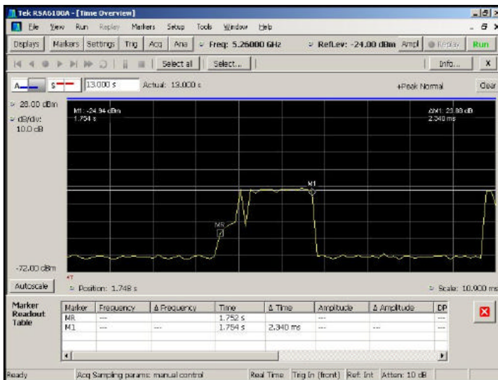
Figure 5-10. Wide traffic pulse from grouping 3
