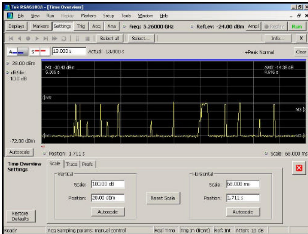
Figure 5-9. Traffic pulse grouping 3
