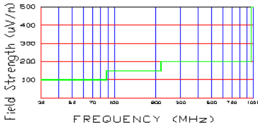
Figure 6-1. 3-Meter Limits
