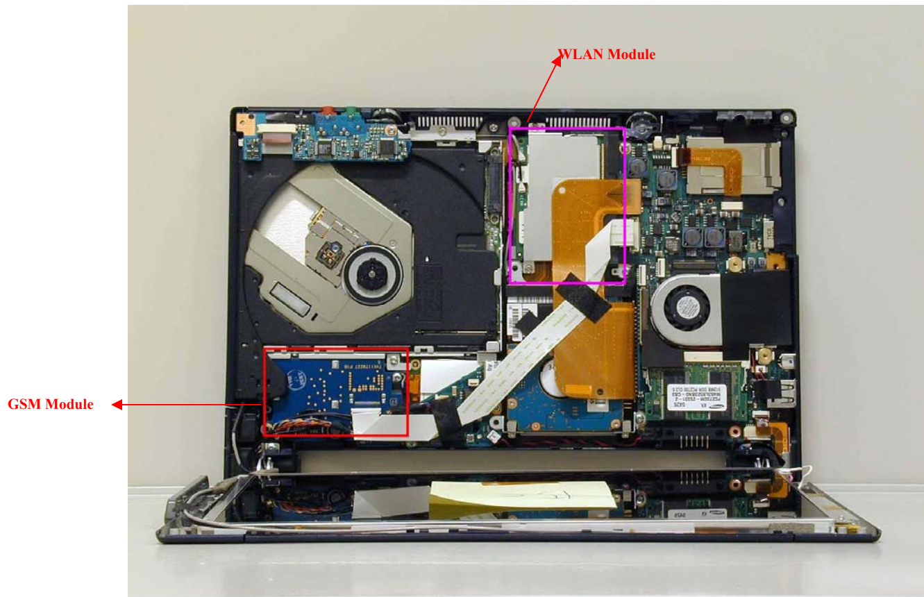
Laptop Internal view showing location of WLAN and GSM modules
