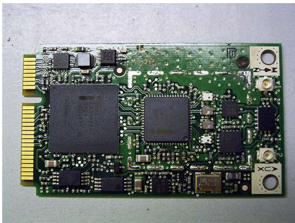
WLAN module (Cover off)
