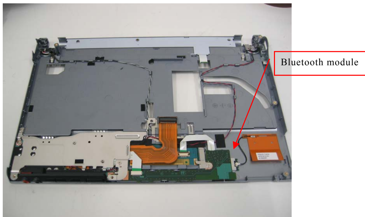
Internal View 2 (Bluetooth module location)
