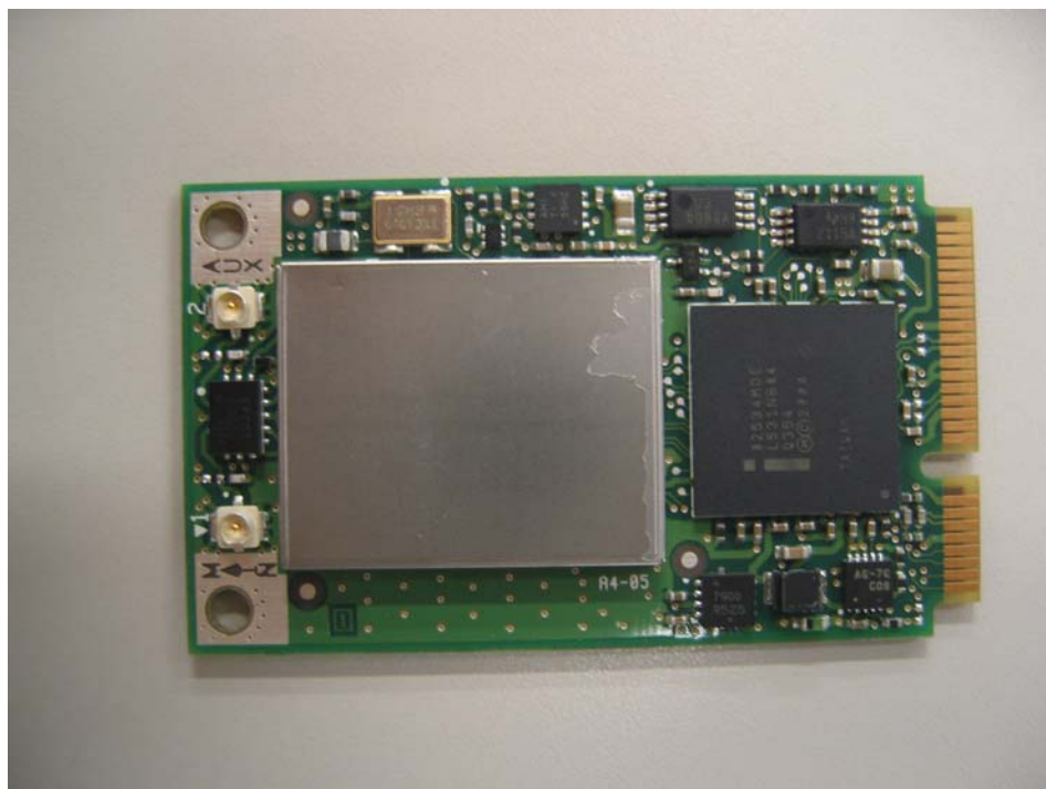
WLAN module (with cover)
