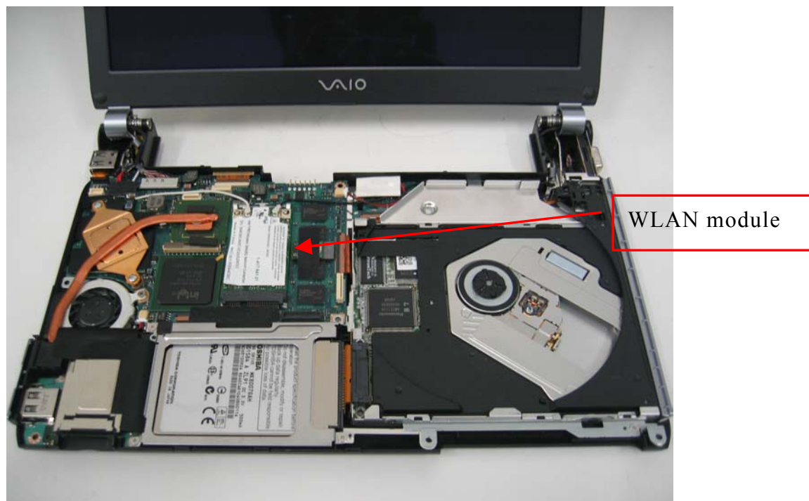
Internal View 1 (WLAN module location)
