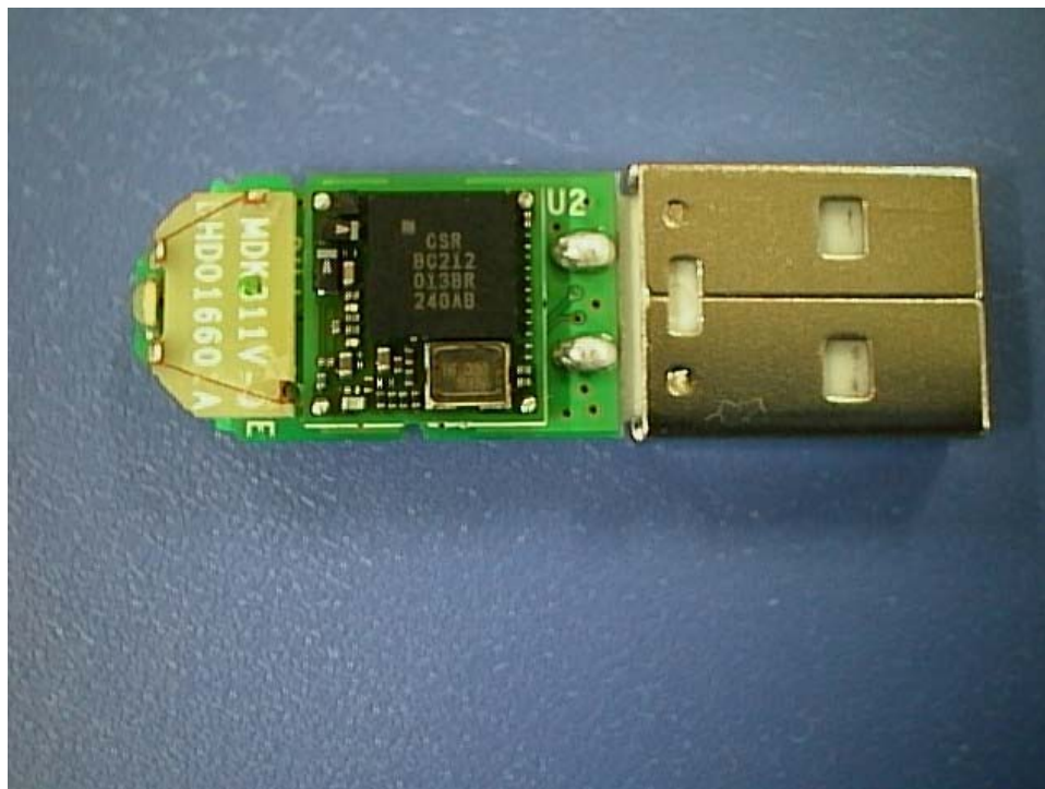
Top View without Cover
