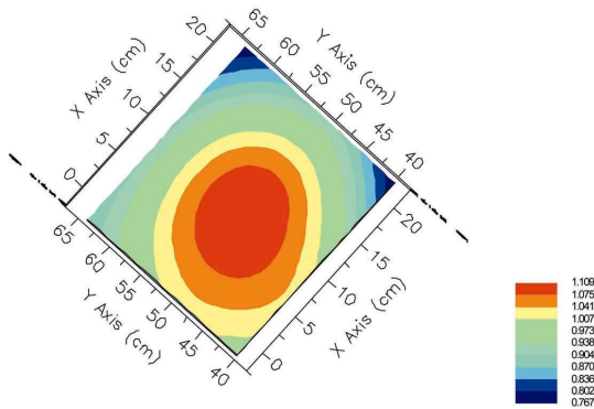
Contour at z=5 mm
