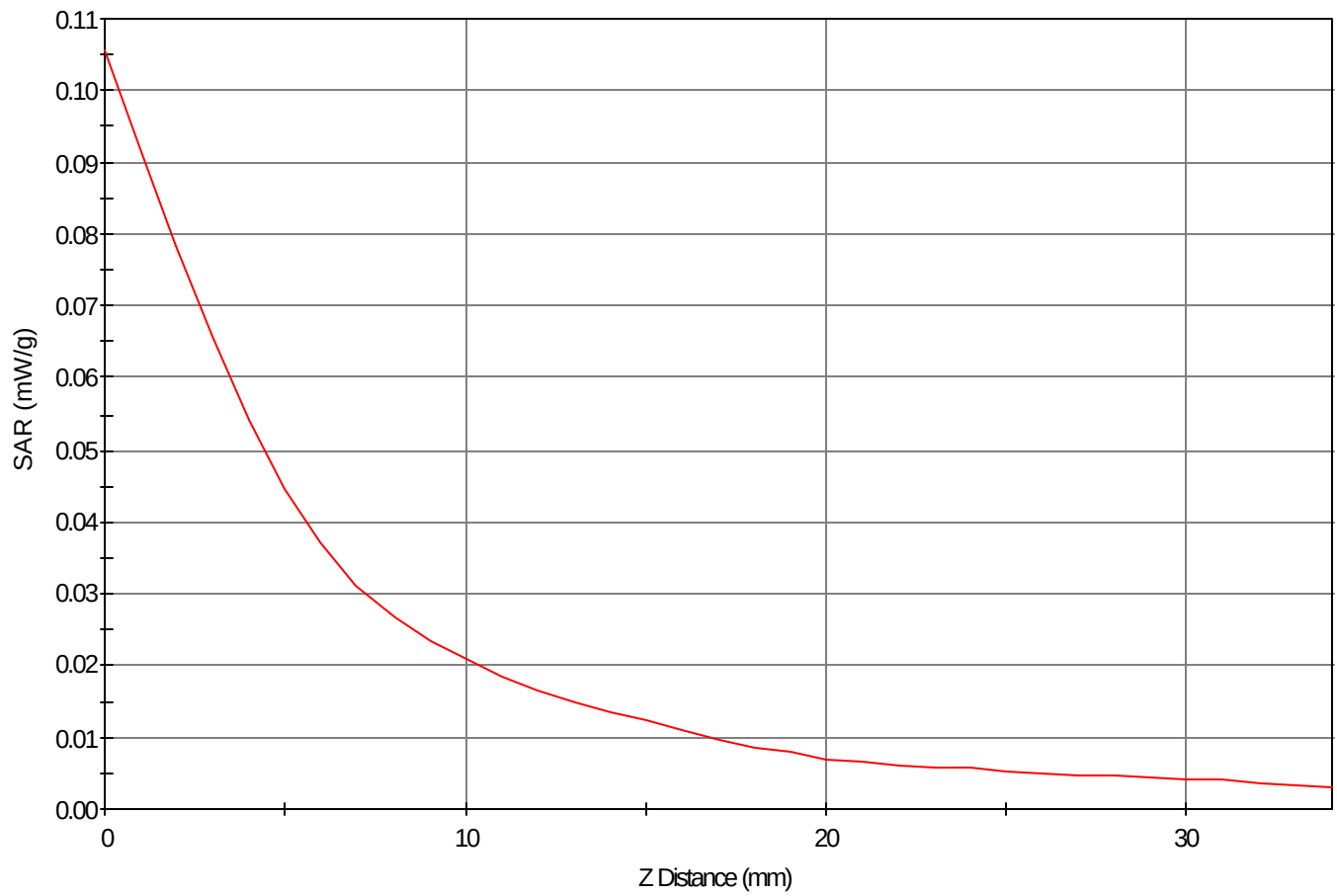
SAR - Z Axis at Hotspot x:-10.0 y:-8.0
