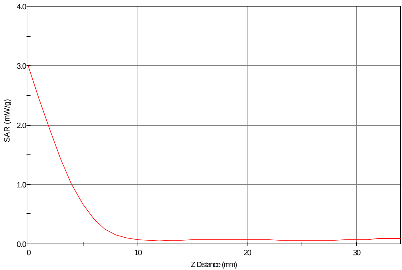
SAR - Z Axis at Hotspot x:-15.0 y:-4.0
