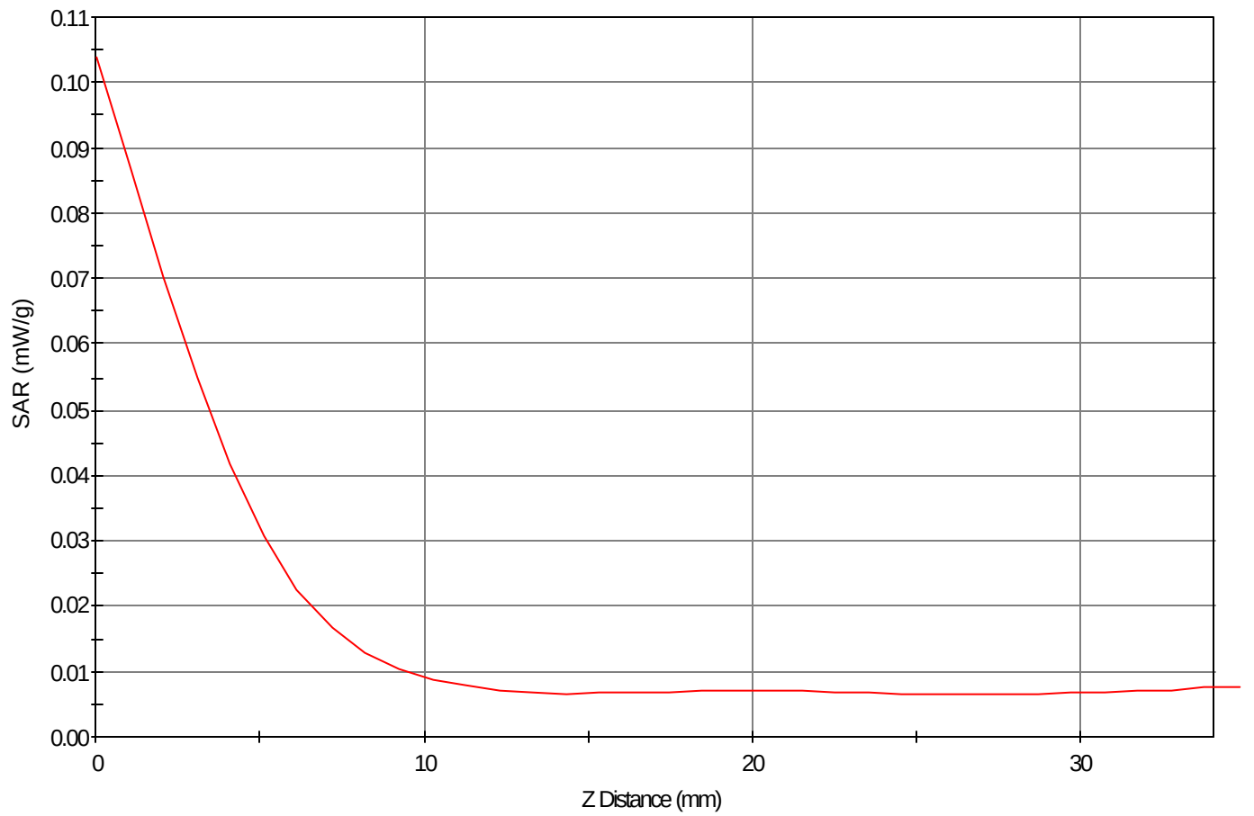
SAR - Z Axis at Hotspot x:-5.0 y:12.0
