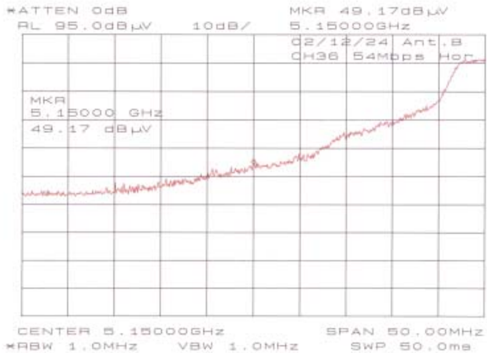
Chart of CH36 with 54Mbps in Antenna B
