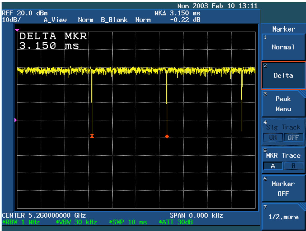
Chart of CH52 with 6Mbps
