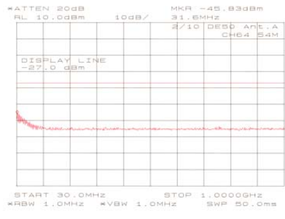
Chart of ch 64 with 54 Mbps in Antenna 1
