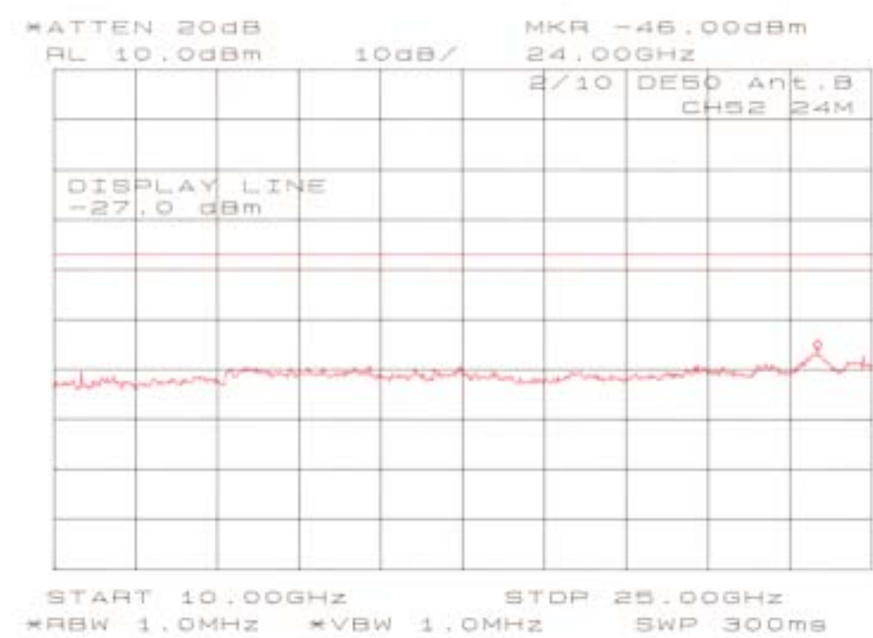
Chart of ch 52 with 24 Mbps in Antenna 2
