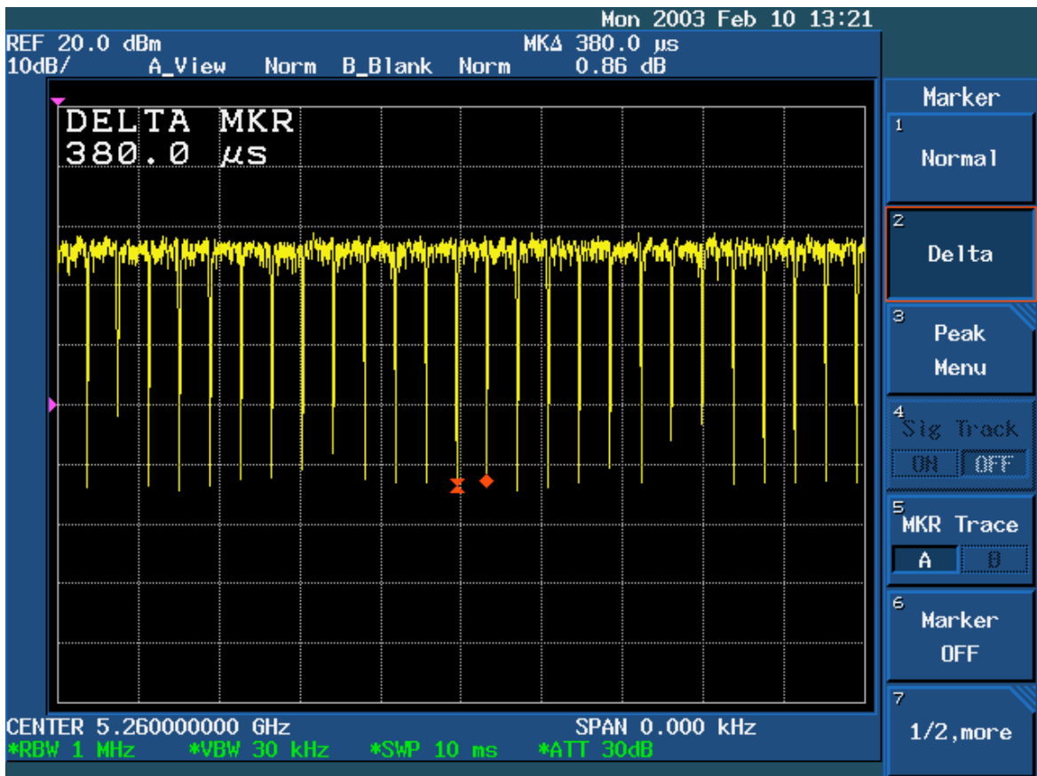
Chart of CH52 with 54Mbps
