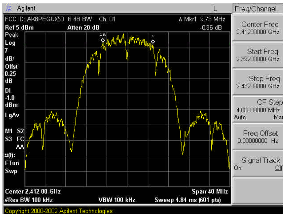
Plot A-1. 6dB Bandwidth Plot – Ch. 01
