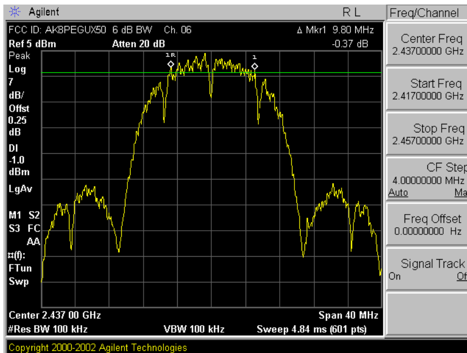
Plot A-2. 6dB Bandwidth Plot – Ch. 06
