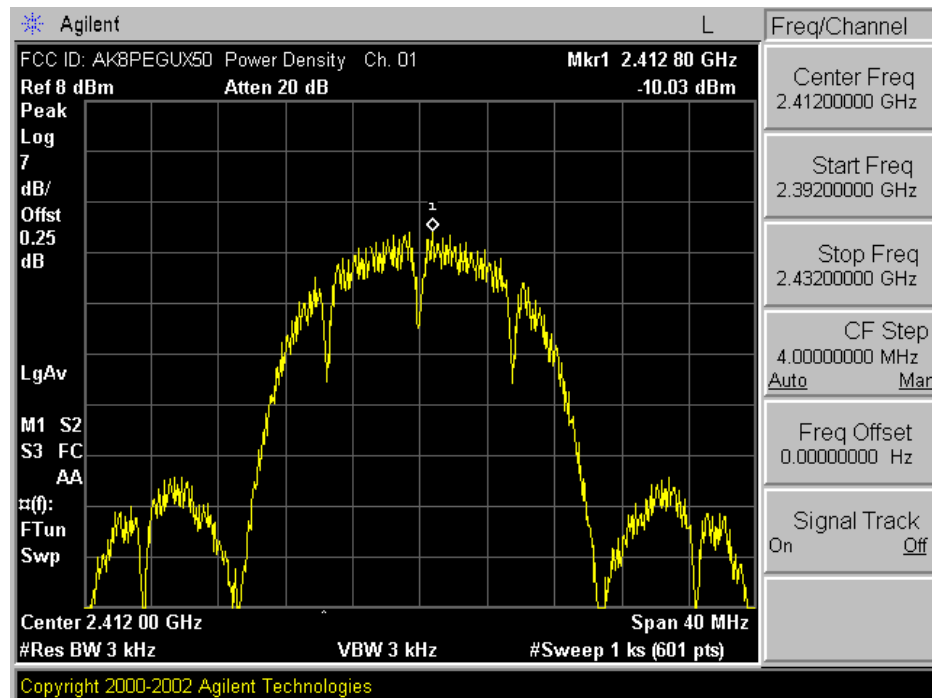
Plot A-7. Max. Power Density Plot – Ch. 01
