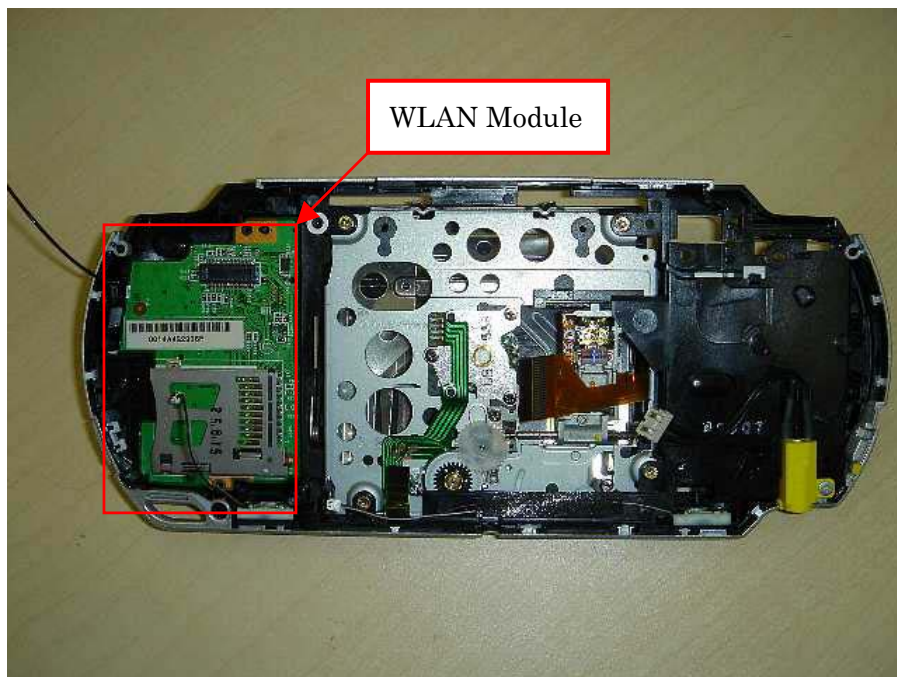
Location of WLAN Module
