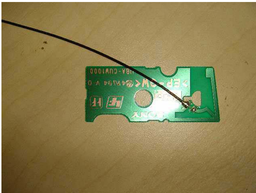
Front View of Antenna (UBA-CUW1000)
