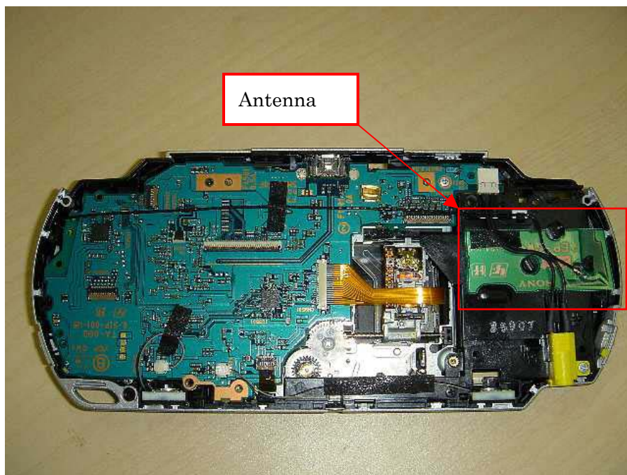
Location of Antenna
