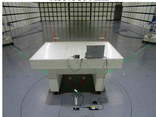
Above 30 MHz
