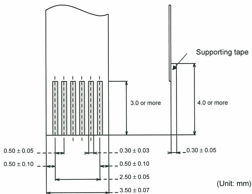
Figure C-1: Recommended FFC/FPC dimensions
