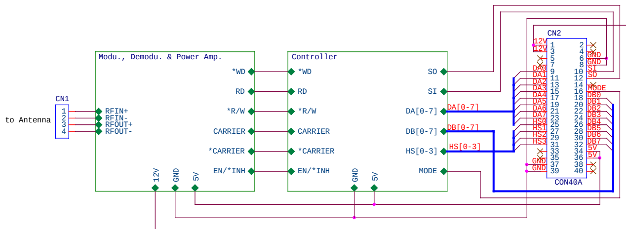
Fig.1 : Pin Assignment of Connectors CN1-2
